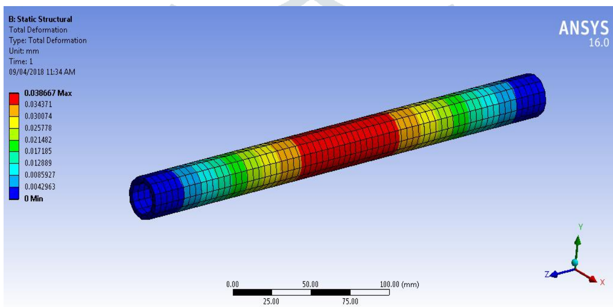
Fig.14 Deformation using Carbon Epoxy Woven Material
