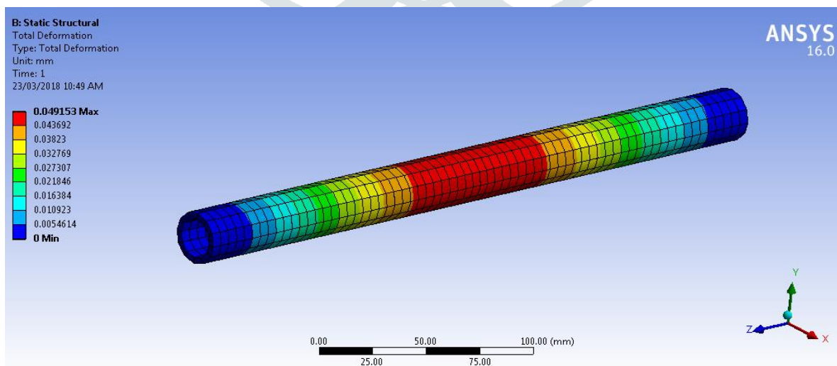
Fig.10 Deformation on shaft
