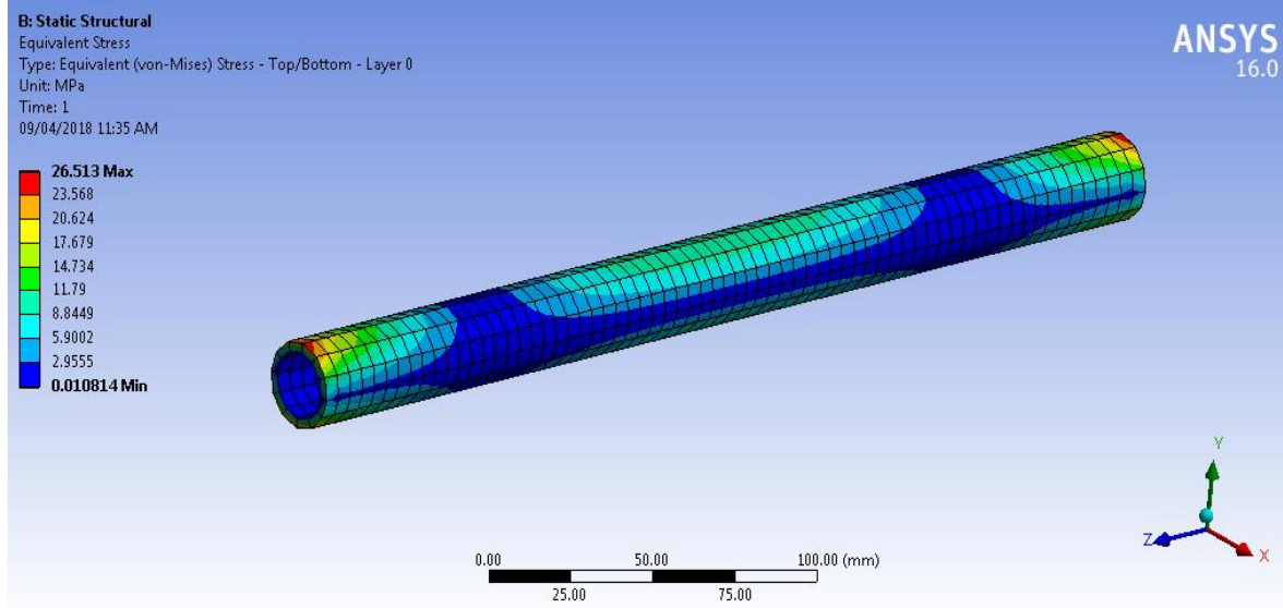
Fig.13 stresses using Carbon Epoxy Woven Material
