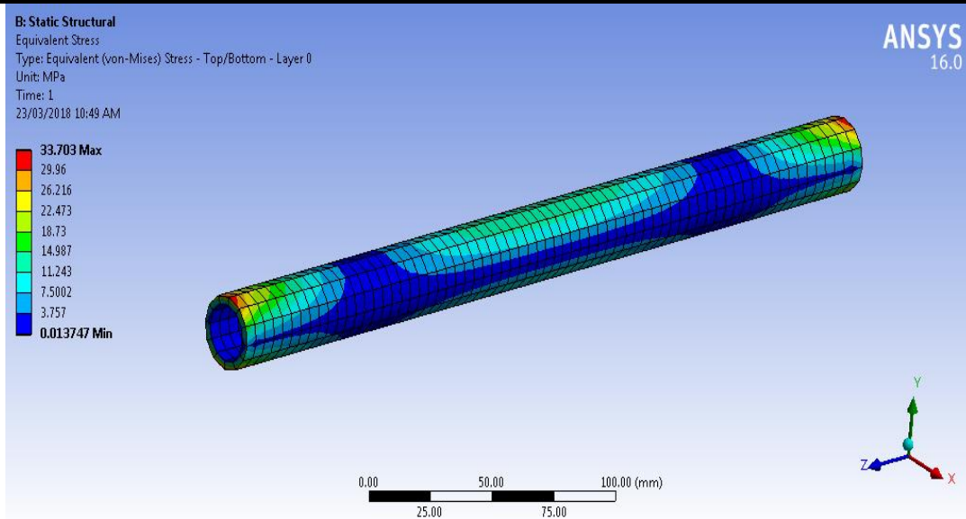
Fig.11. Stresses on shaft
