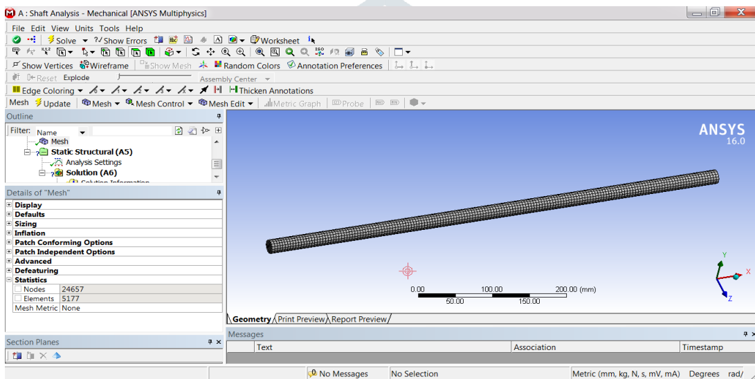
Fig.4 Meshing of the shaft using hexahedral elements
