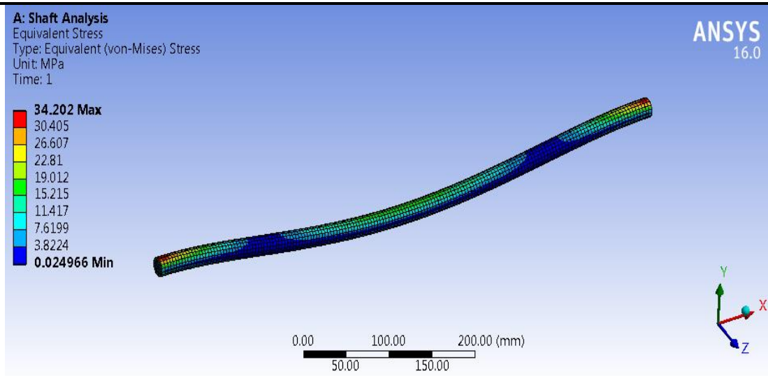
Fig.6 Von Misses Stresses in the shaft
