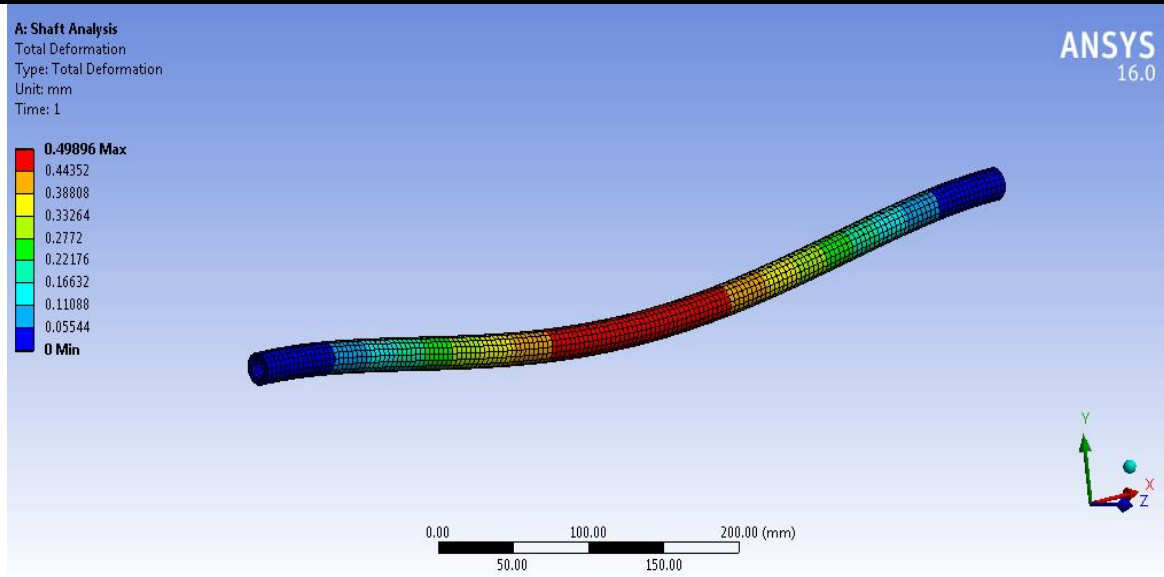
Fig.9 Deformation in hollow shaft
