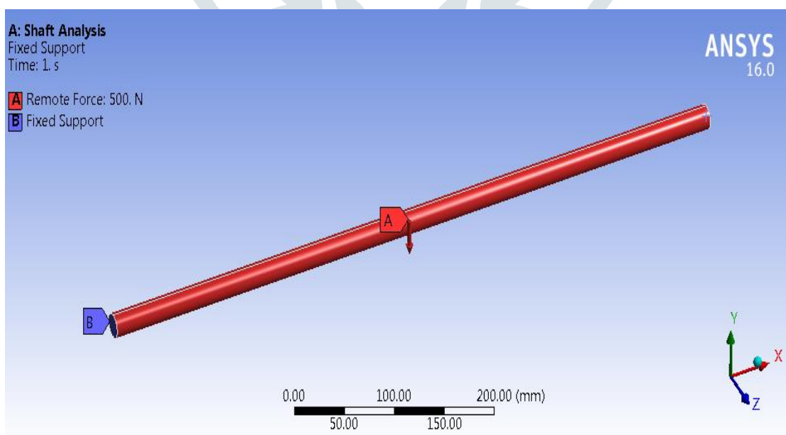
Fig.5 Boundary condition on shaft
