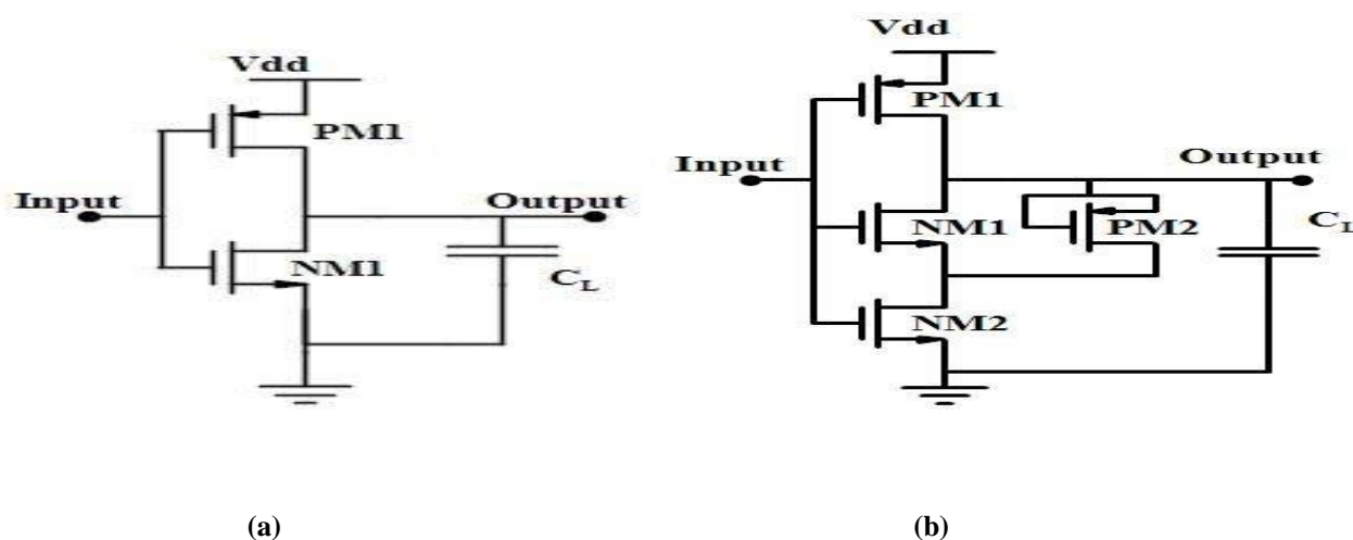
Fig. 2. Circuit schematic of CMOS inverter designed using: (a) Conventional technique, (b) proposed technique.
