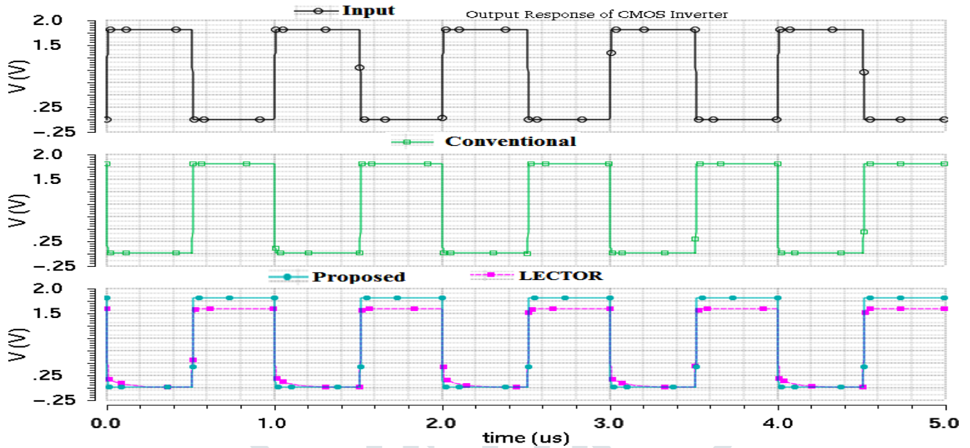
Fig. 6. Output waveforms of CMOS inverter circuit.
