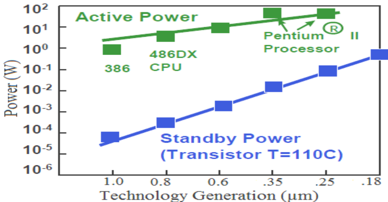
Fig. 1. Power consumption of Intel technologies
