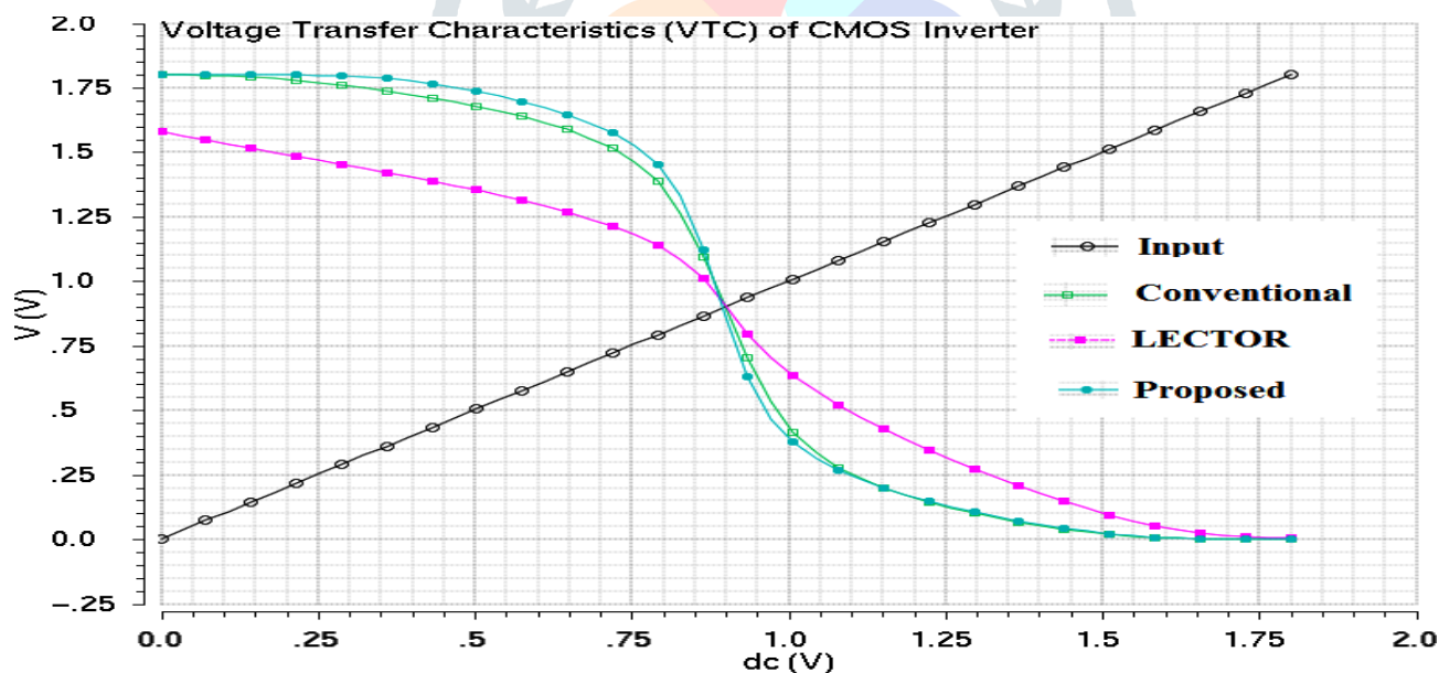
Fig. 5. Voltage Transfer characteristic (VTC) of CMOS Inverter circuit
