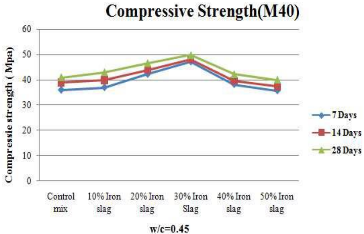
Figure 1: Compressive strength of iron slag concrete.
