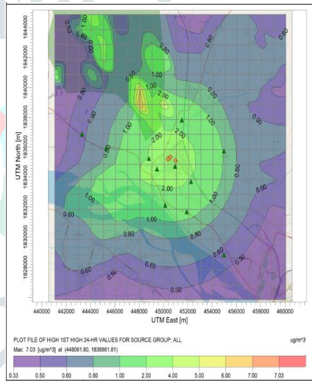
Isopleths for 24hr SPM concentration
