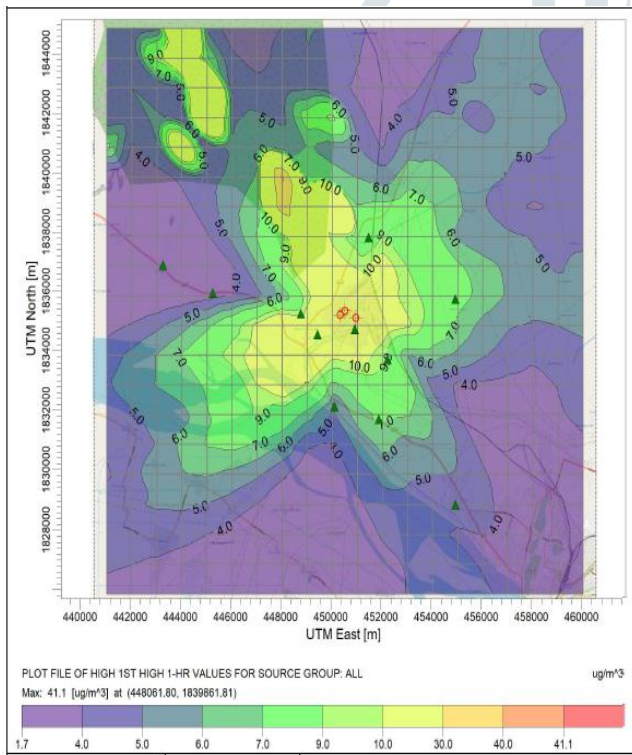
Isopleths for 1hr SPM concentration
