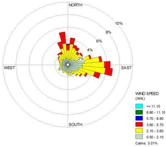
Surface file wind rose
