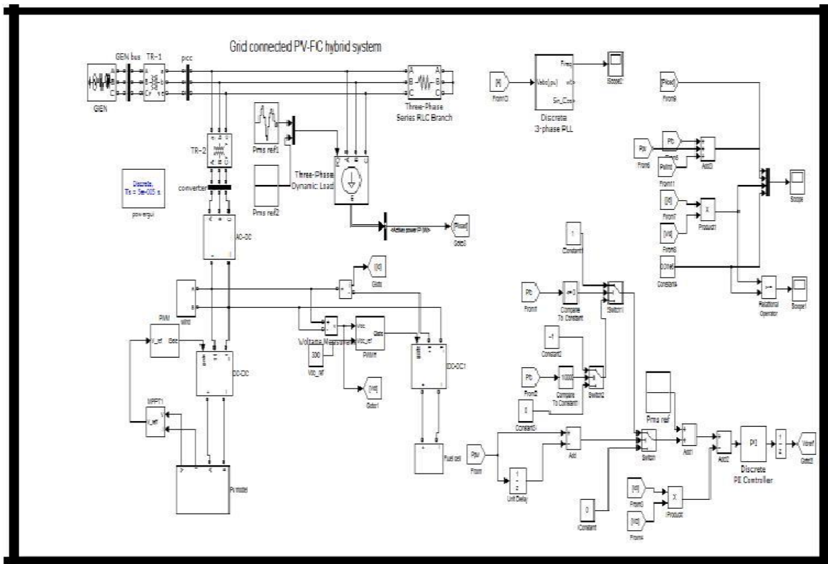
Fig 10- Grid connected operating strategy of the whole system
