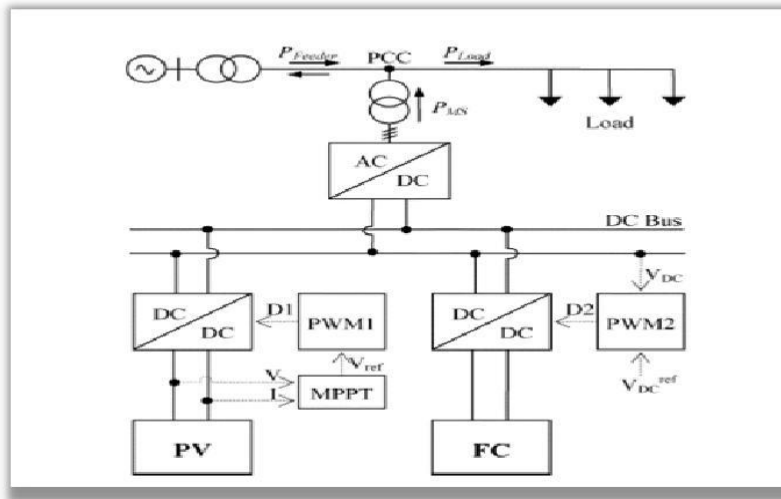
Fig 5-PV-FC base grid connected system
