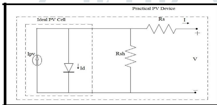
Fig 7: Equivalent circuit of a practical PV device [6]
