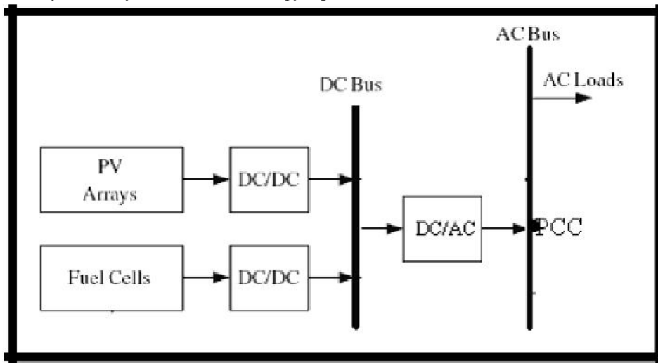
Fig-1-Grid connected PV-FC Hybrid system
