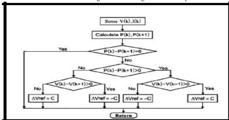
Fig 6-P & O algorithm
