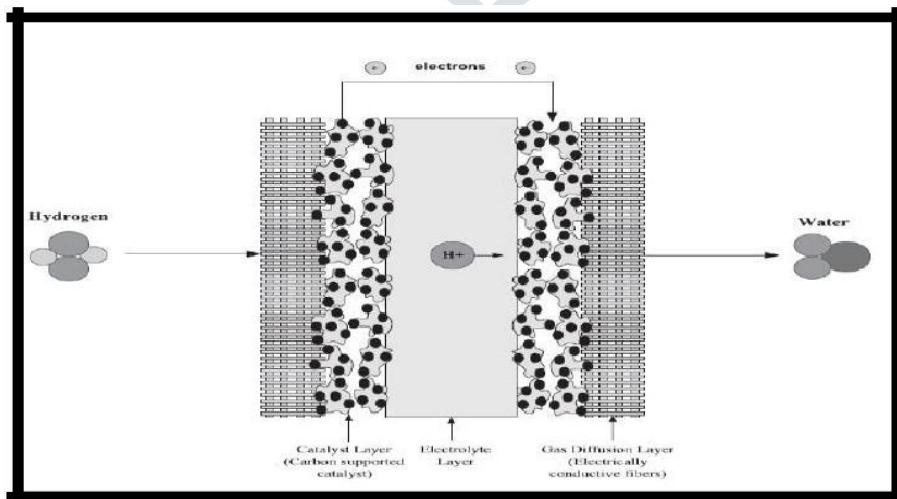
Fig 4-A single PEM fuel cell configuration
