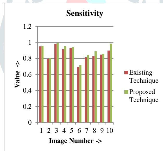
Fig 4.2: Sensitivity Analysis
