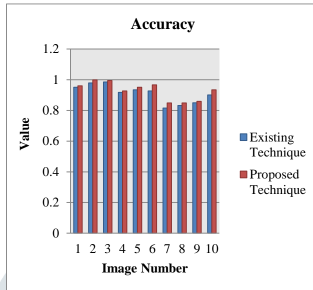
Fig4.1: Accuracy Analysis
