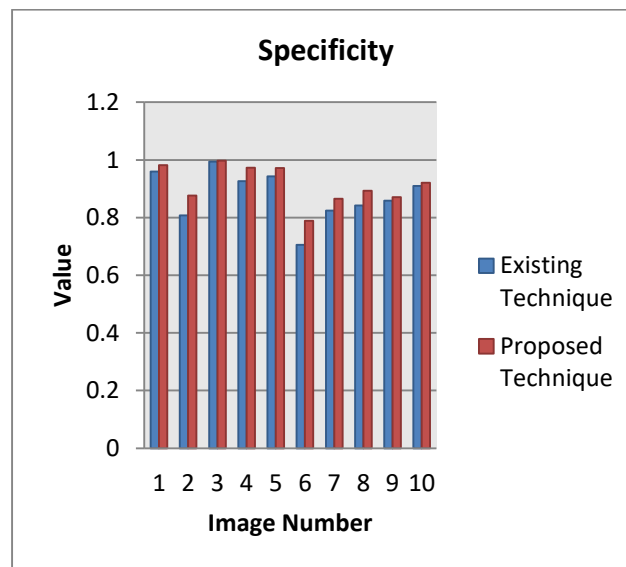
Fig 4.3: Specificity Analysis
