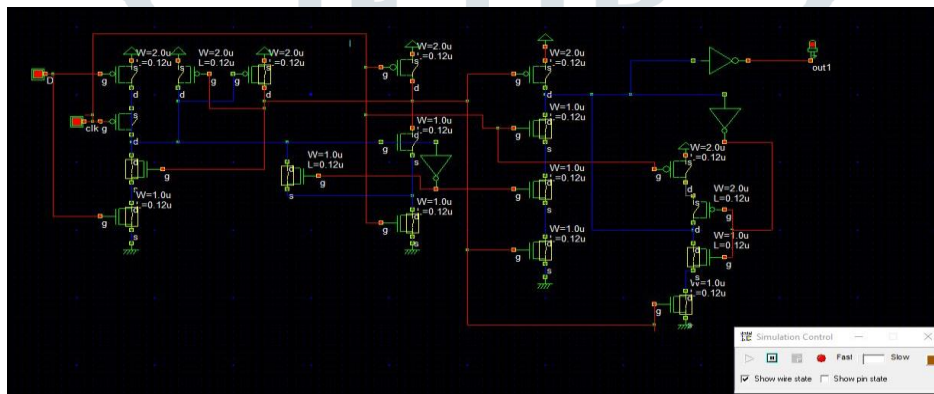
Figure 4: Proposed 18-transistor single-phase clocked (TSPCFF)
