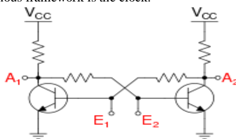
Figure 1: A traditional (simple) flip-flop circuit based on bipolar junction transistors
