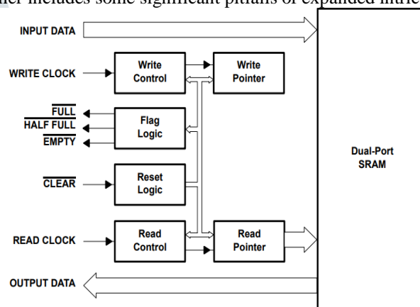
Figure 2: Block diagram of FIFO with storage
