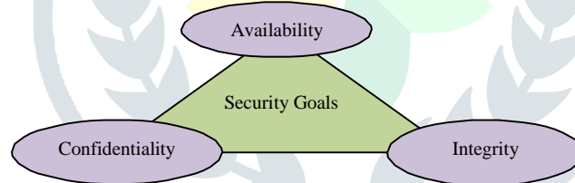
Figure 6. Security Goals
