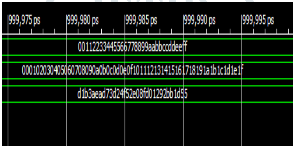
Figure 5: Encryption Process
