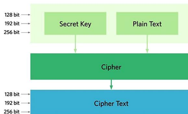
Figure 1: AES Model
