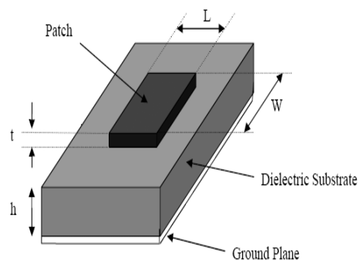
Figure 2.1 Basic Geometry of Microstrip Patch Antenna
