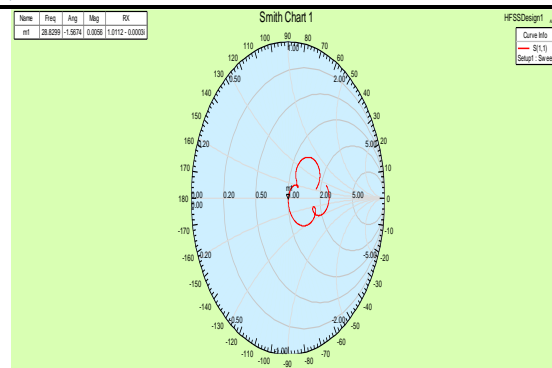
Figure 4.3 Smith Chart
