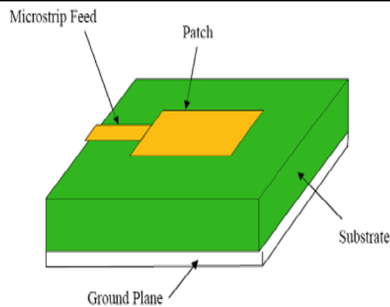
Figure 2.2 Microstrip line feed
