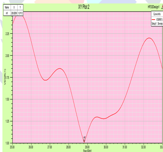
Figure 4.2 VSWR Plot
