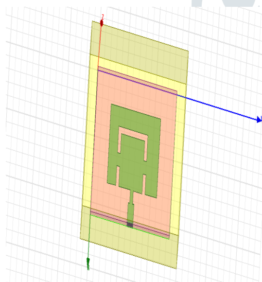
Figure 3.1 Proposed UWB Antenna Design (Top View)
