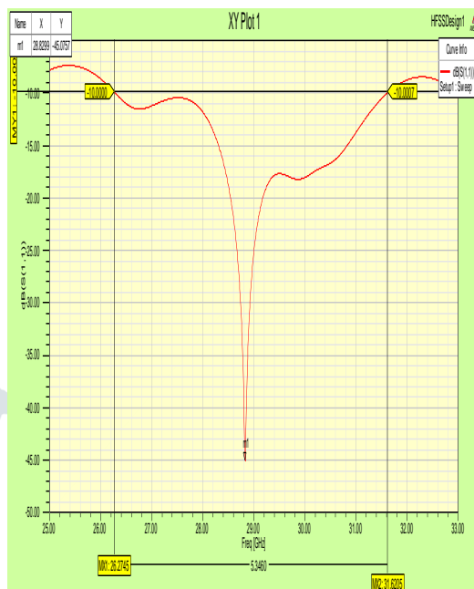
Figure 4.1 S-Parameter
