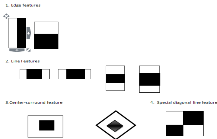
Figure 3: Cascade classifier
