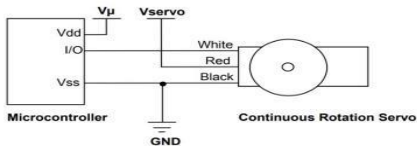
Figure 2: Servo
