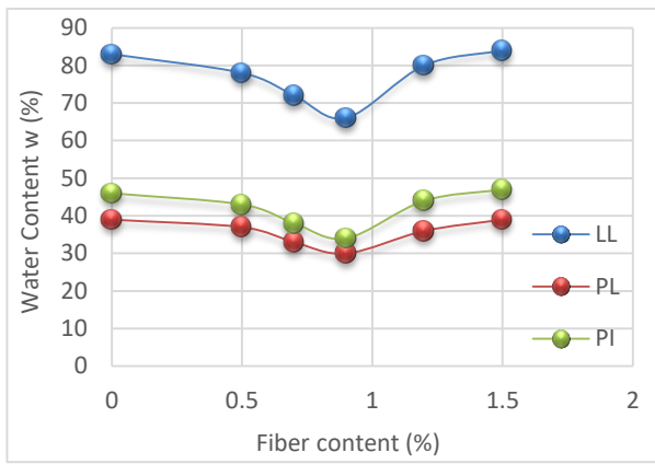
Fig 4:Variation of Consistency Limits
