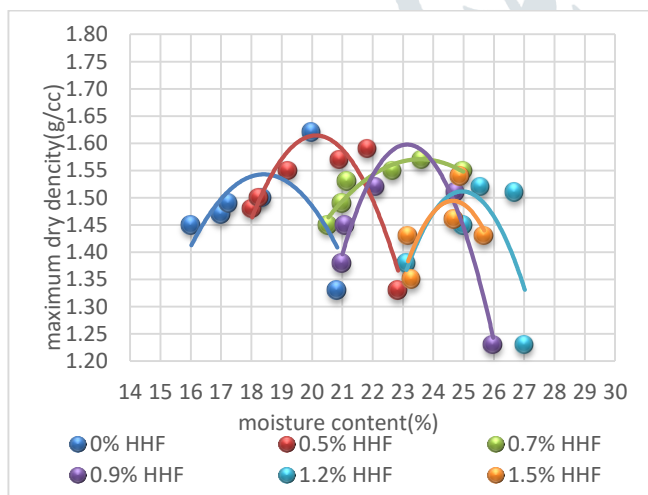
Fig 5:Moisture content vs Dry density for HHF Admixed soil
