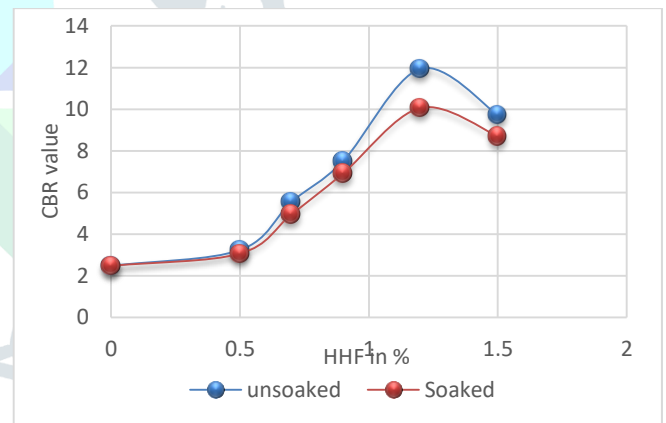
Fig 8:CBR values for un-soaked and soaked conditions for HHF admixed soil
