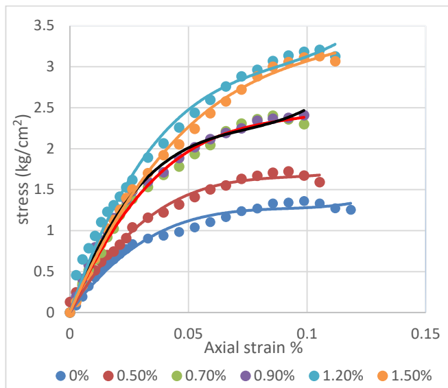
Fig 10: Stress vs Strain
