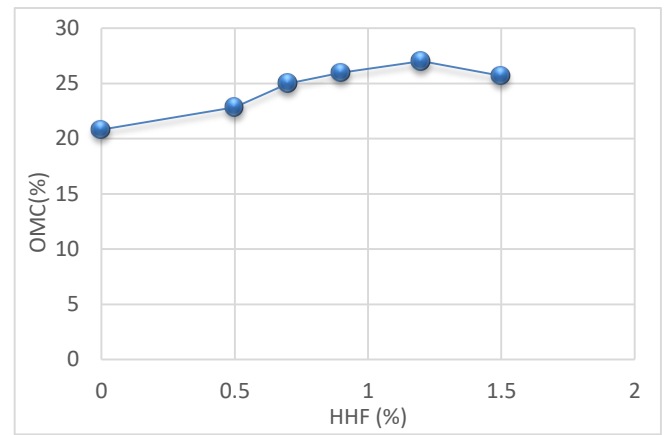
Fig 6:HHF% vs Corresponds optimum moisture content
