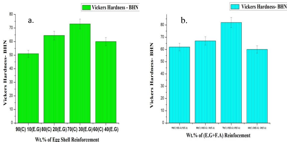
Fig. 3.a. Brinell Hardness Test results for Egg shell reinforcement in to Cork
