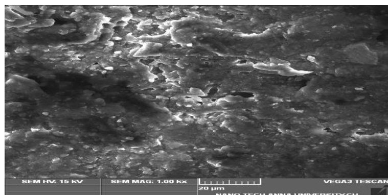
c. Cork+Egg shell+Fly Ash(70%+15%+15%) composites
