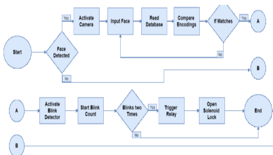
Figure 2.2-System Process Overview
