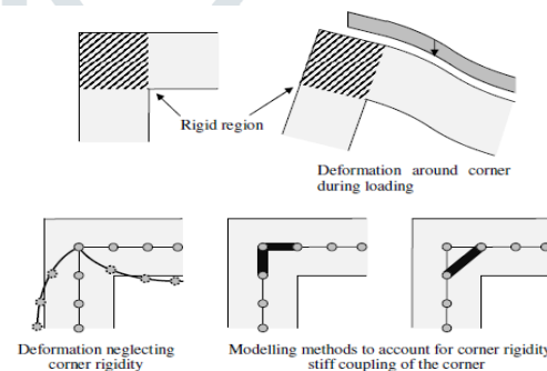
Response of a frame corner during loading and the response of a model neglecting frame corner rigidity. Alternative models for accounting frame corner rigidity are also shown,
