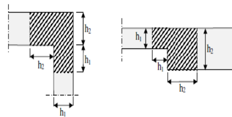
Examples of discontinuity regions, D-regions, where the strain distribution will differ from the linear strain distribution predicted by beam theory. The extent of the discontinuity is often assumed to be equal to the width of the element.
