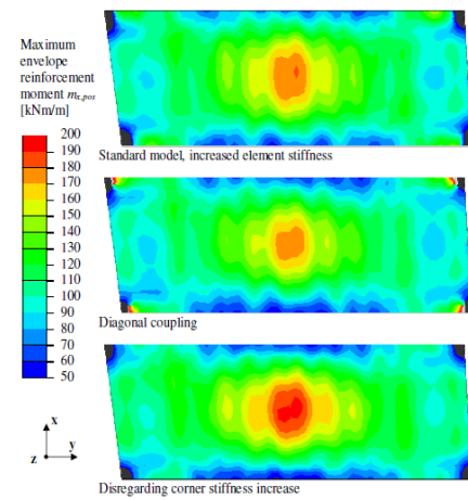
Maximum envelope reinforcement moment in the bridge deck (resisted by bottom reinforcement). Corner stiffness modelled with increased material stiffness (top), corner nodes in the critical sections coupled diagonally (middle) and corner stiffness increase neglected (bottom). Local peak values due to torsion near the slabs corners are not shown.
