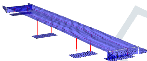
Example of finite element structural analysis model of a double beam bridge. Beam elements shown as lines (red) represent main beams and columns, shell elements shown as surfaces (blue) represent bridge deck, end shields, wing walls and foundation slabs.
