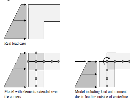
Different models for bookkeeping stacking outside of centre lines.
