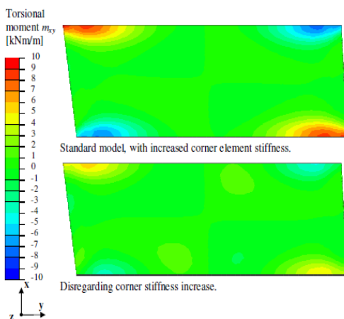
Difference in torsional moment in the bridge deck for load case self-weight. The model neglecting support stiffness (bottom) shows substantially lower torsional moment near the deck corners than the models accounting for support stiffness (top).
