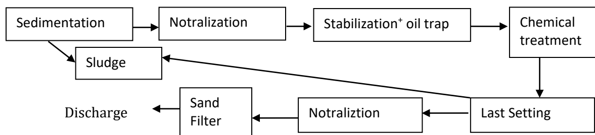
Fig. 1. In enamel industry, refining plant flow sheet for physico-chemical refining
