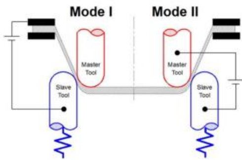
Figure 1: Schematic diagram of the circuit connection in E-DSIF
