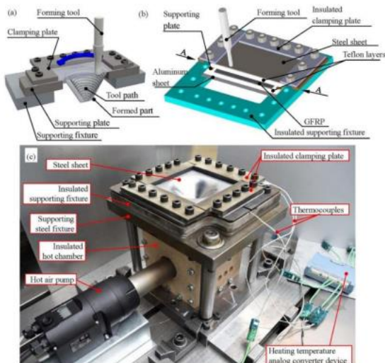
Figure 2: Principle of SPIF, work piece combination
