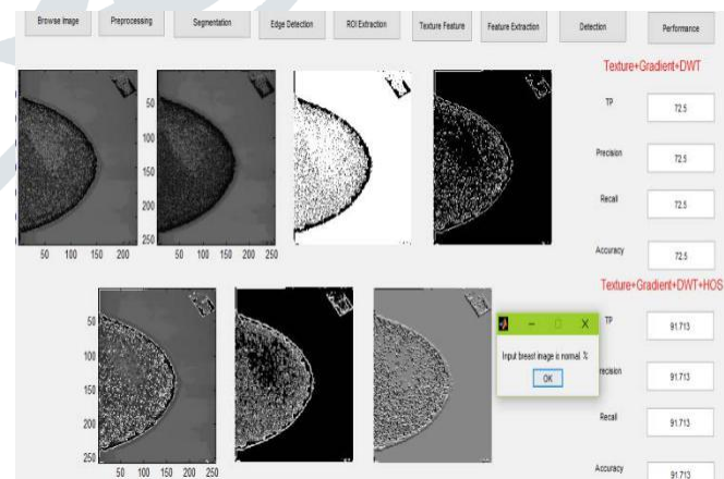
Fig. 2. GUI for proposed framework of automatic detection of cardio vascular based on input cardio image
