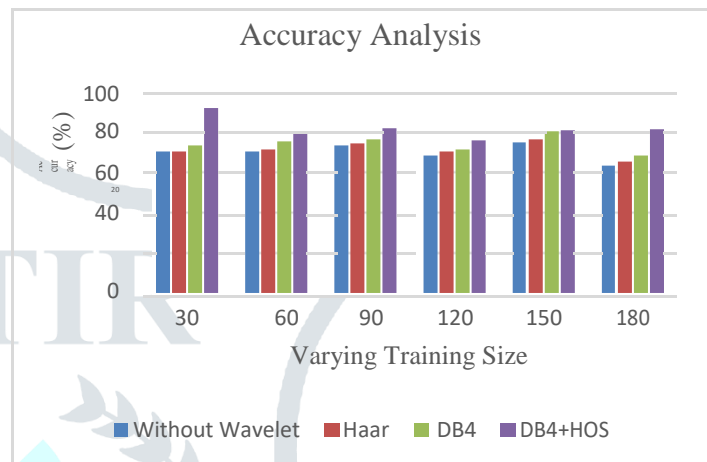
Fig. 3. Comparative analysis of different CAD methods
