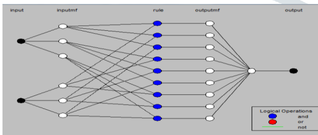
Fig.4: ANFIS-based MPPT structure
