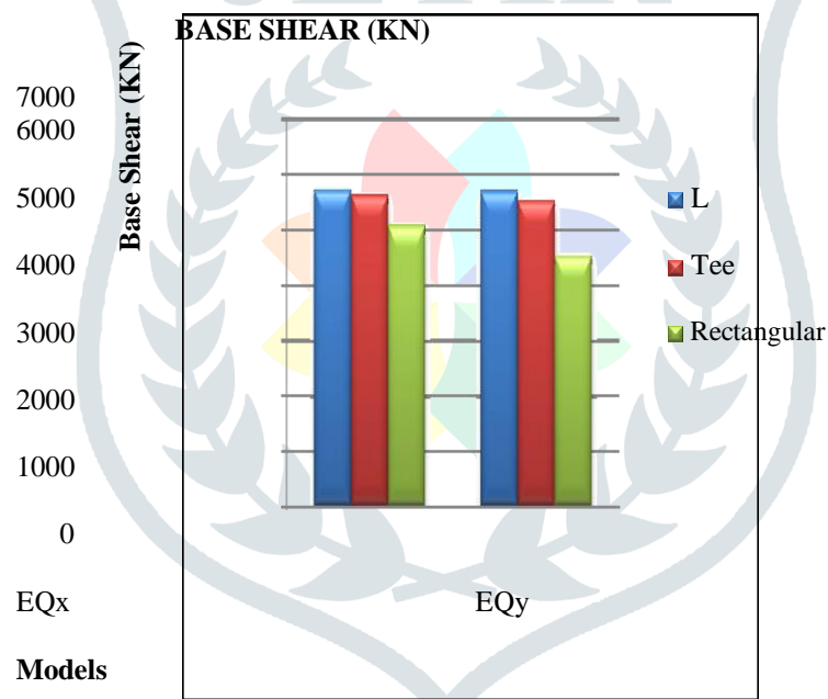
Figure 4: The base shear or lateral forces
