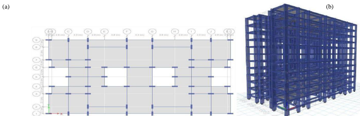
Figure 3: G+10 RCC Framed Structure with Rectangular Column c/s (a) Plan (b) 3D View
