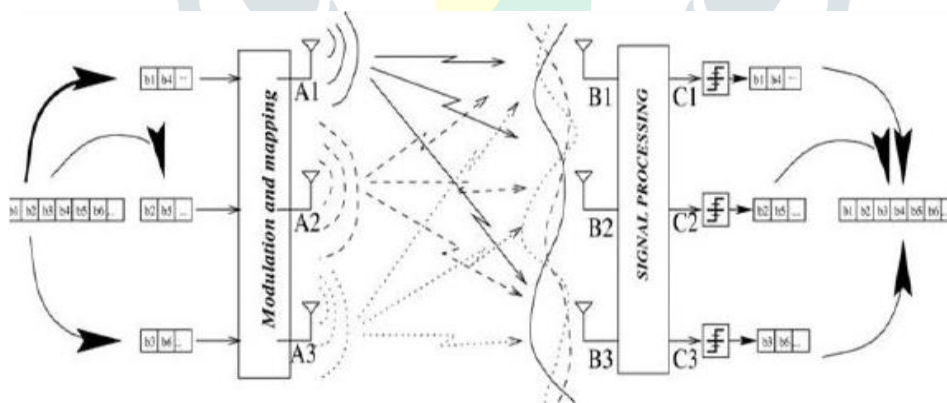
Fig 1.4.4: BLAST architecture
