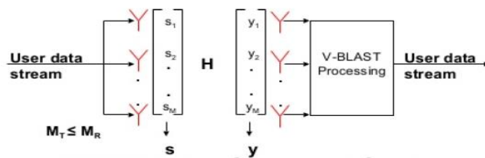
Fig 1.4.4.2: V-BLAST architecture
