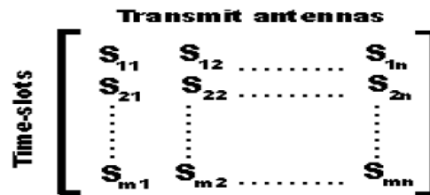
Fig 1.4.1: Space-time block code matrix representation
