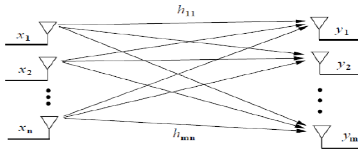
Fig 1.1 : MIMO systems
