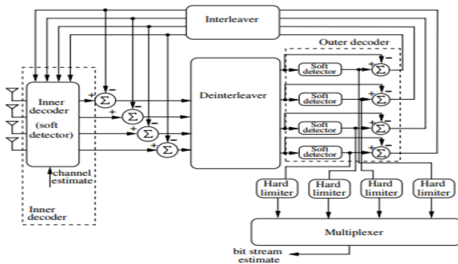
Fig 1.4.4.3.2: Decoder of Turbo BLAST architecture
