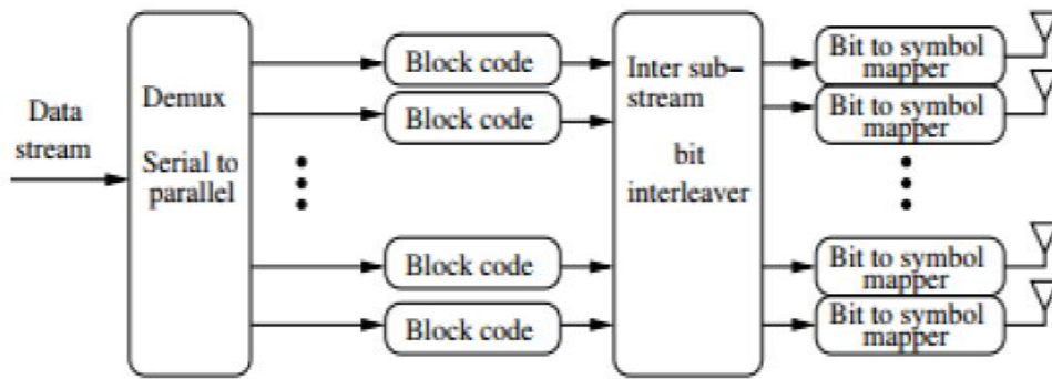
Fig 1.4.4.3.1: Encoder of Turbo BLAST architecture
