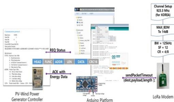
Fig.3. Arduino based IoT sensor platform
