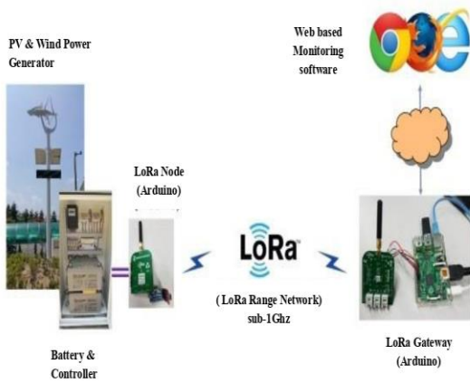
Fig.2. Energy monitoring system architecture
