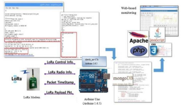
Fig.4. Arduino base monitoring system
