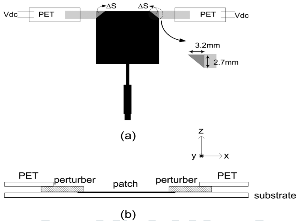
Fig 4. Diagram of the proposed antenna (a) Top view and (b) Side view
