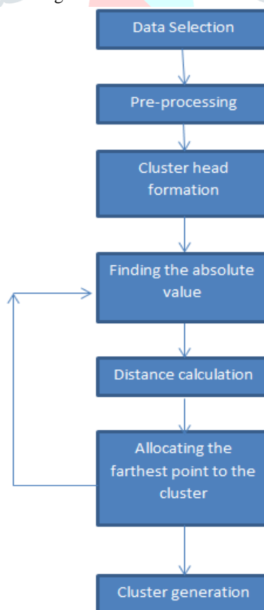
Fig (3) Architecture Diagram
