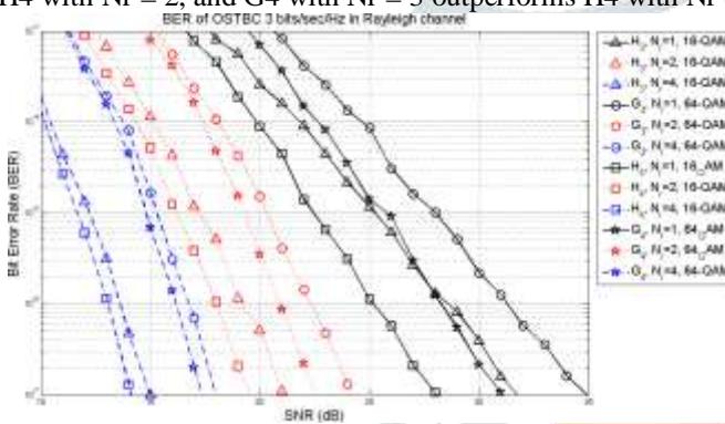
Figure 5 Bit error rate versus SNR of OSTBC at 3 bits/sec/Hz.
