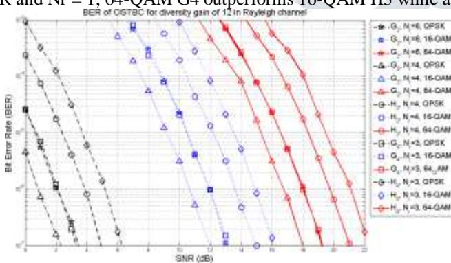
Figure 6. Bit error rate versus SNR of OSTBC with spatial diversity 12.
