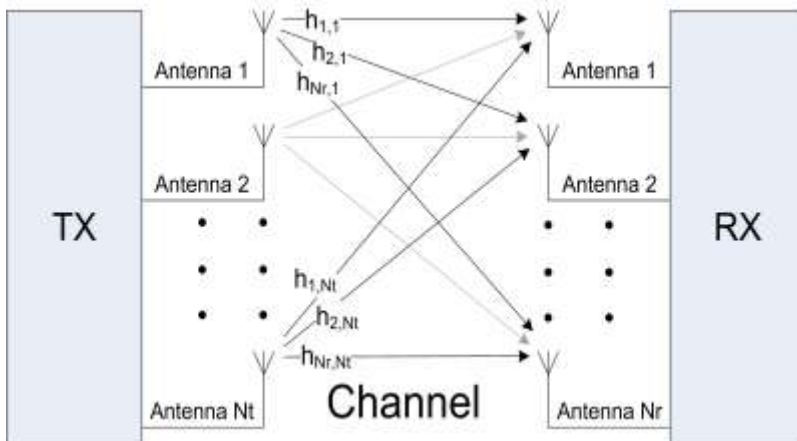
Figure1. Multiple-Input Multiple-Output system block diagram.
