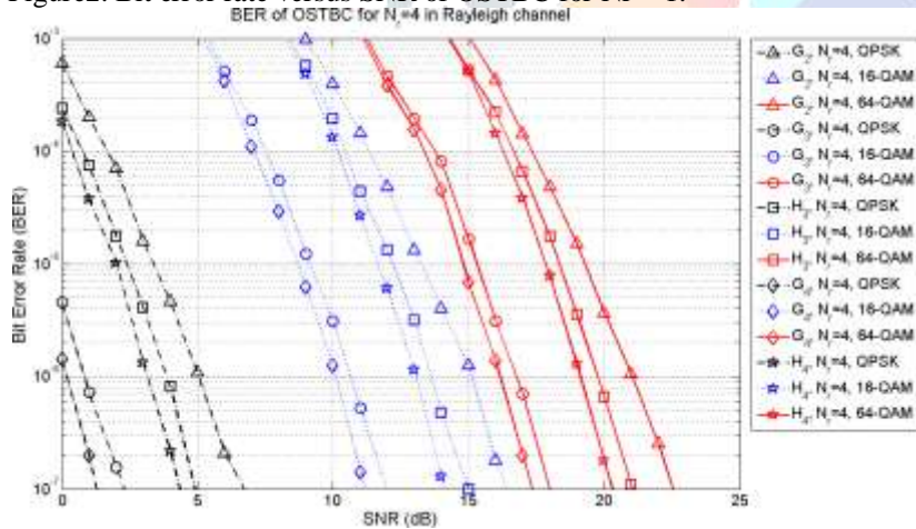
Figure3. Bit error rate versus SNR of OSTBC for N_r = 4 .
