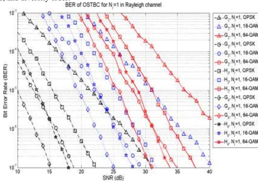
Figure2. Bit error rate versus SNR of OSTBC for N_r = 1 .
