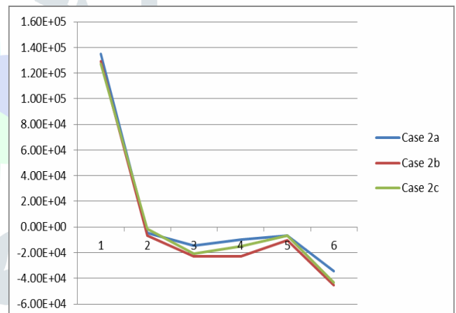
Story Drift in X & Z Direction
