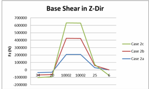
No. Of Nodes Vs Base Shear in Z Direction Story Drift in X & Z Direction
