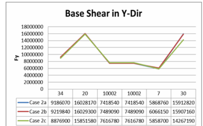
No. Of Nodes Vs Base Shear in Y Direction
