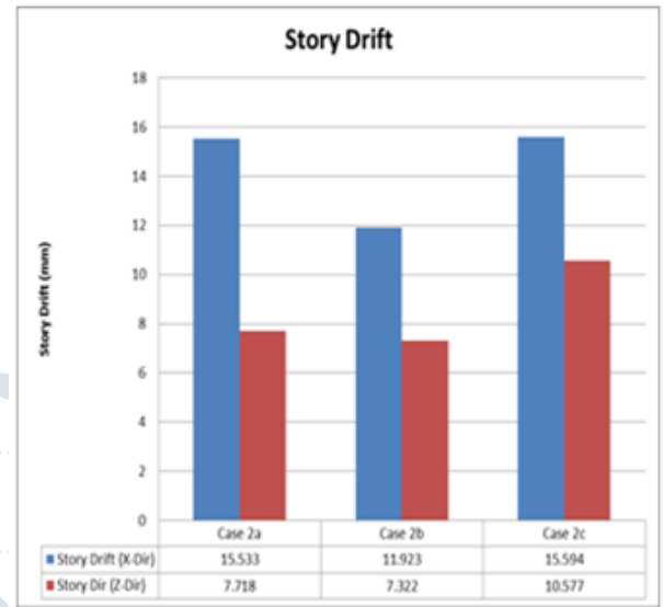
Story Drift in X & Z Direction
