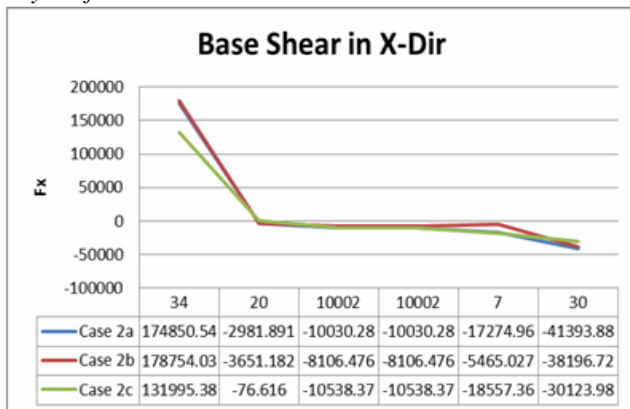
No. Of Nodes Vs Base Shear in X Direction
