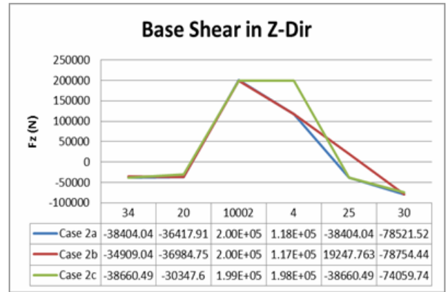
No. Of Nodes Vs Base Shear in Z Direction
