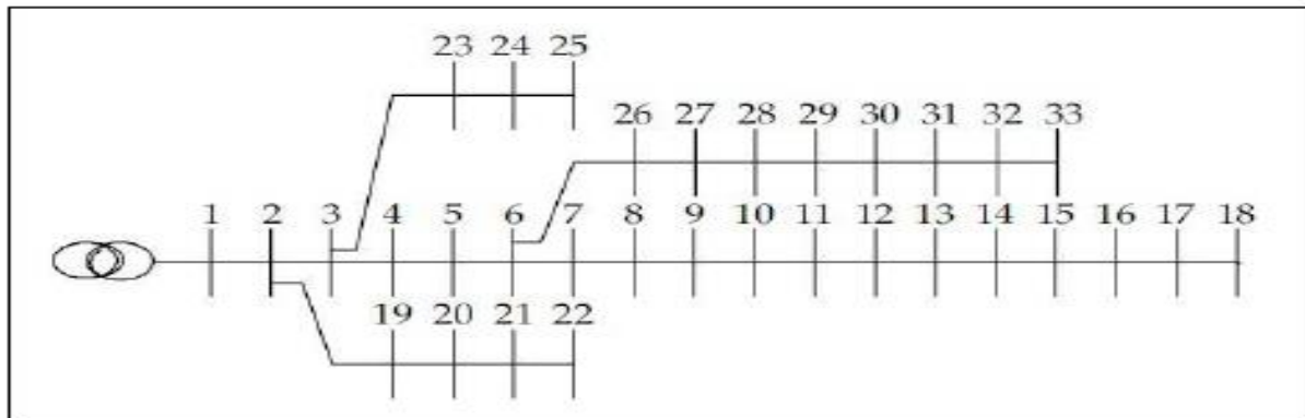
Fig.3.1: Single diagram of IEEE 33 bus test system
