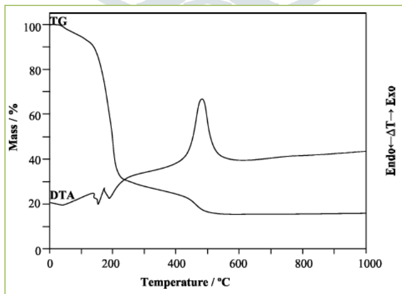
Fig.4. TG and DTA curves of the [\text{Cu}(\text{en})_2(\text{H}_2\text{O})]_2[\text{SiW}_{12}\text{O}_{40}] complex
