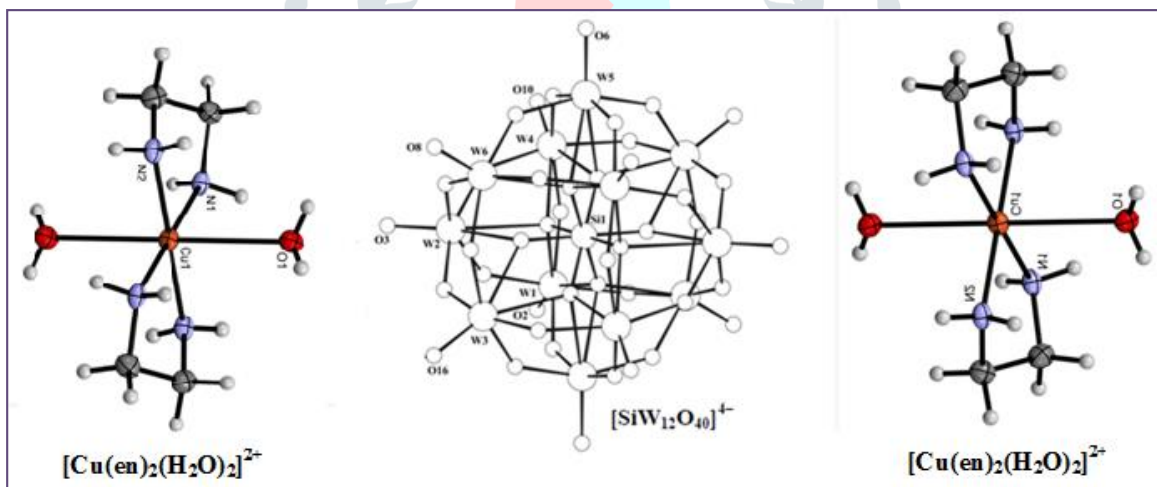
Fig.1a. Ortep diagram of one formula unit of [\text{Cu}(\text{en})_2(\text{H}_2\text{O})_2]_2[\text{SiW}_{12}\text{O}_{40}] where Displacement ellipsoids are drawn at the 50% probability level.
