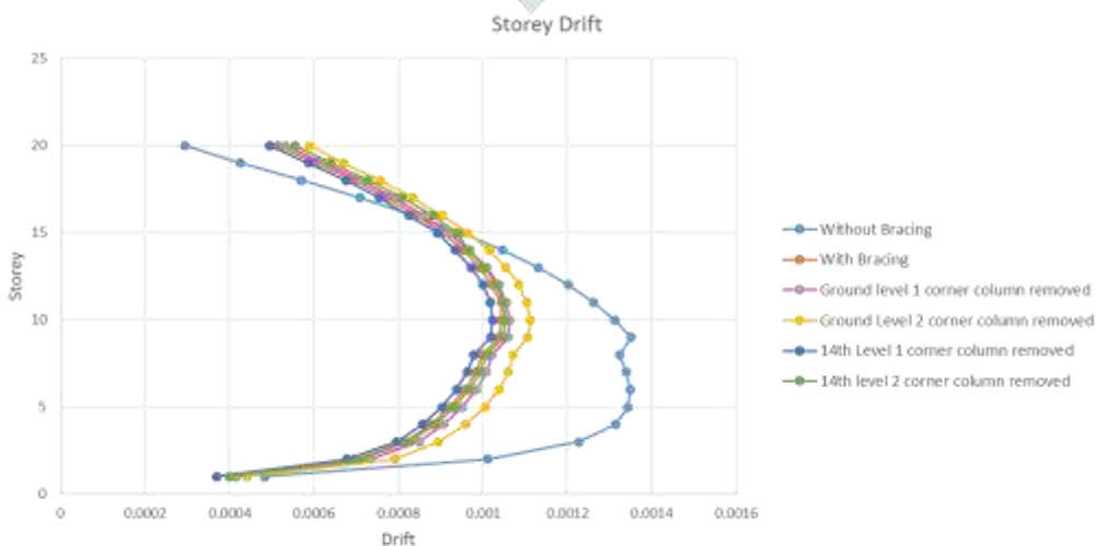
Chart -2: Storey Drift
