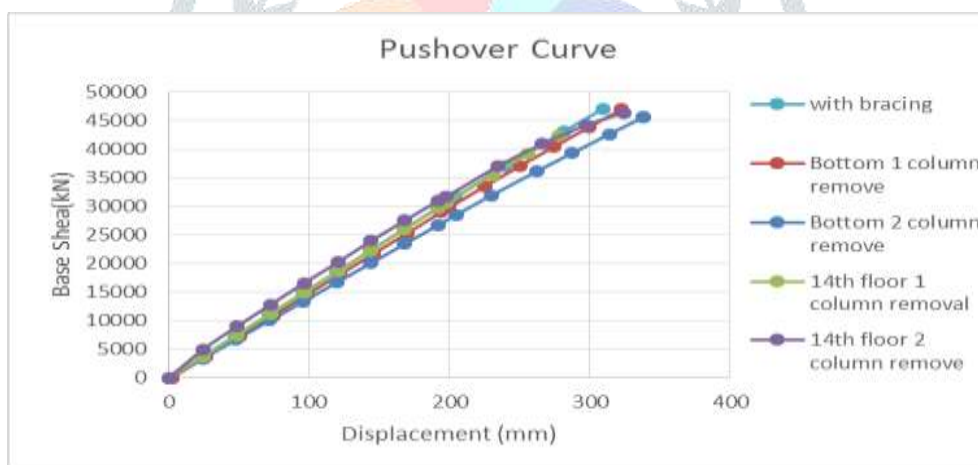
Chart -4: Pushover Curve
