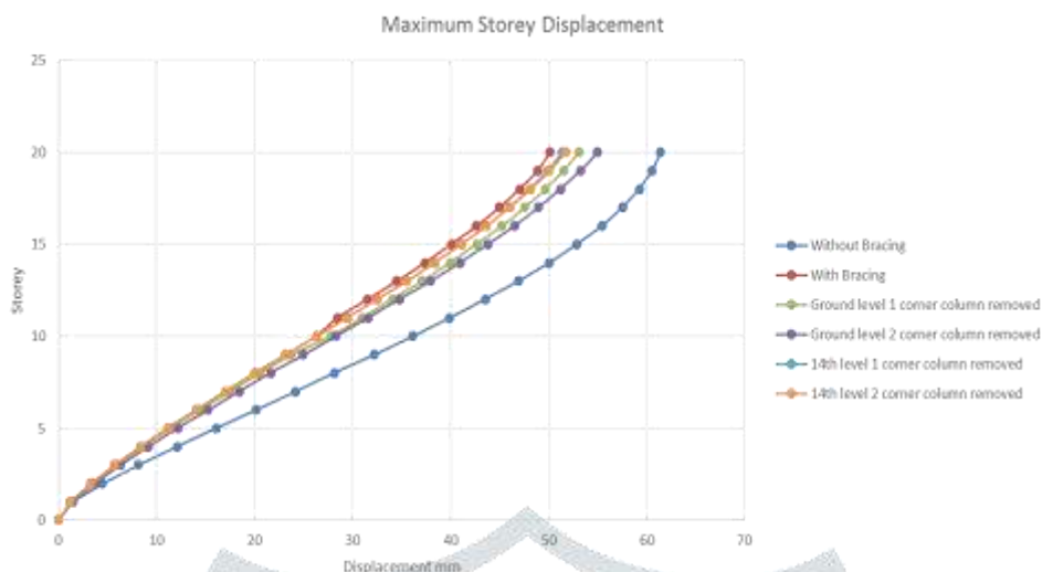
Chart -3: Maximum Storey Displacement
