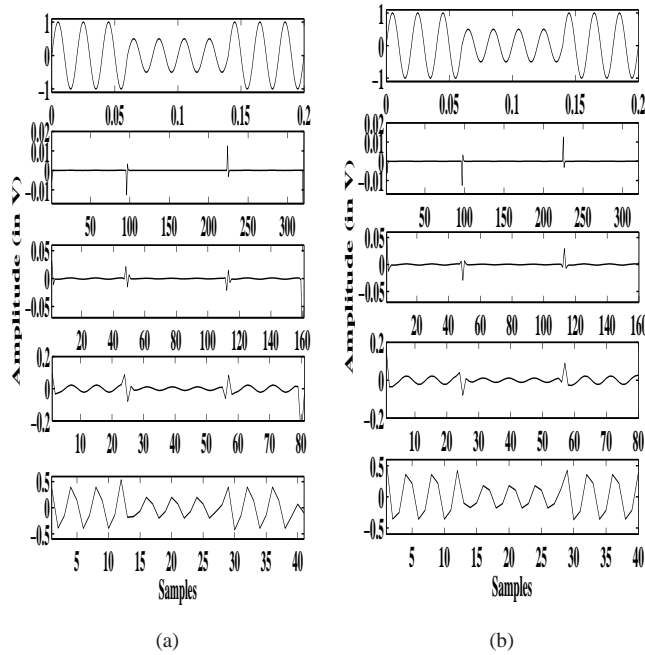
Fig. 4: Localization of sine wave with sag in (a) DWT decomposition (b) SGWT decomposition
