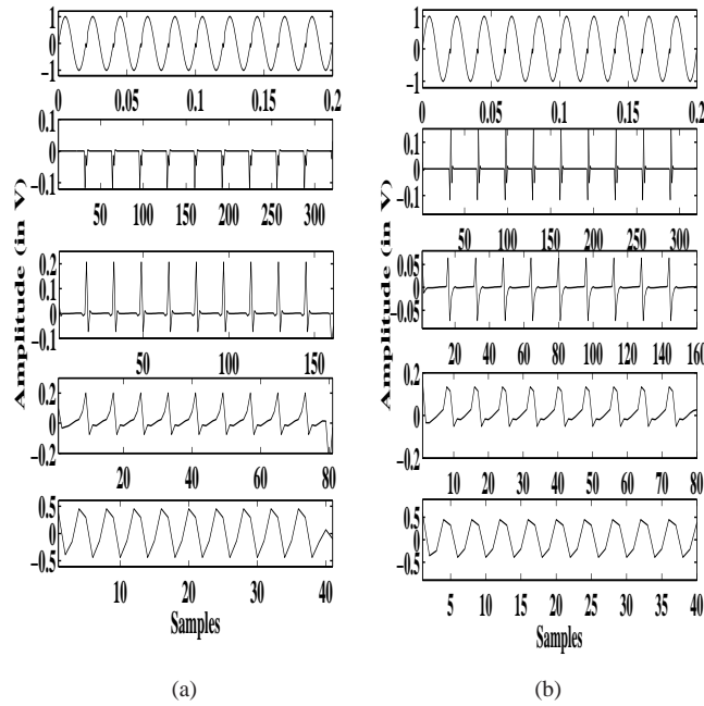
Fig. 8: Sine wave with Harmonic and sag (a) DWT decomposition (b) SGWT decomposition
