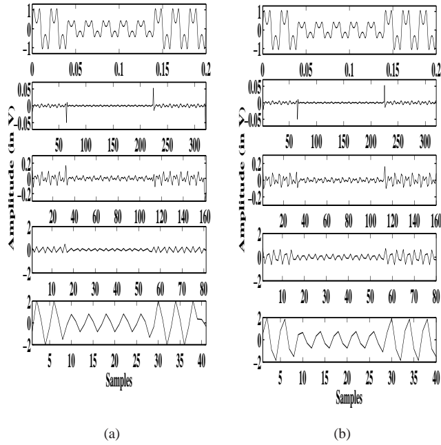
Fig. 7: Sine wave with Harmonic and sag (a) DWT decomposition (b) SGWT decomposition
