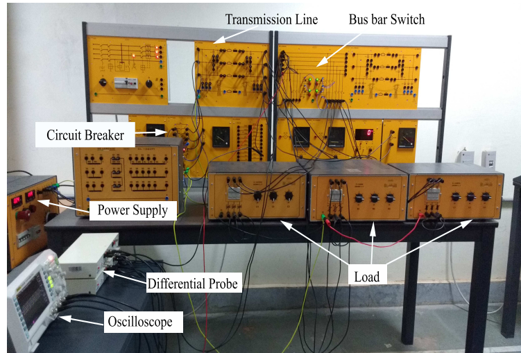
Fig. 9: Experimental setup for three phase voltage signal collection
