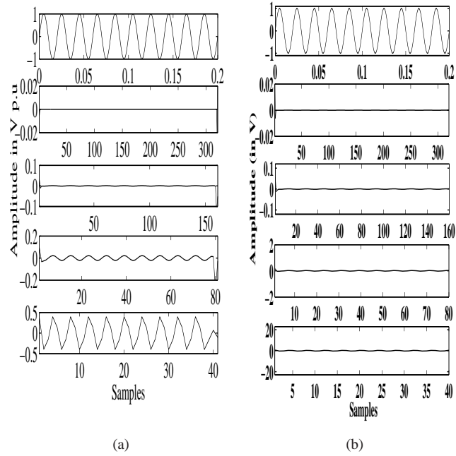
Fig. 3: Localization of pure sine wave in (a) DWT decomposition (b) SGWT decomposition
