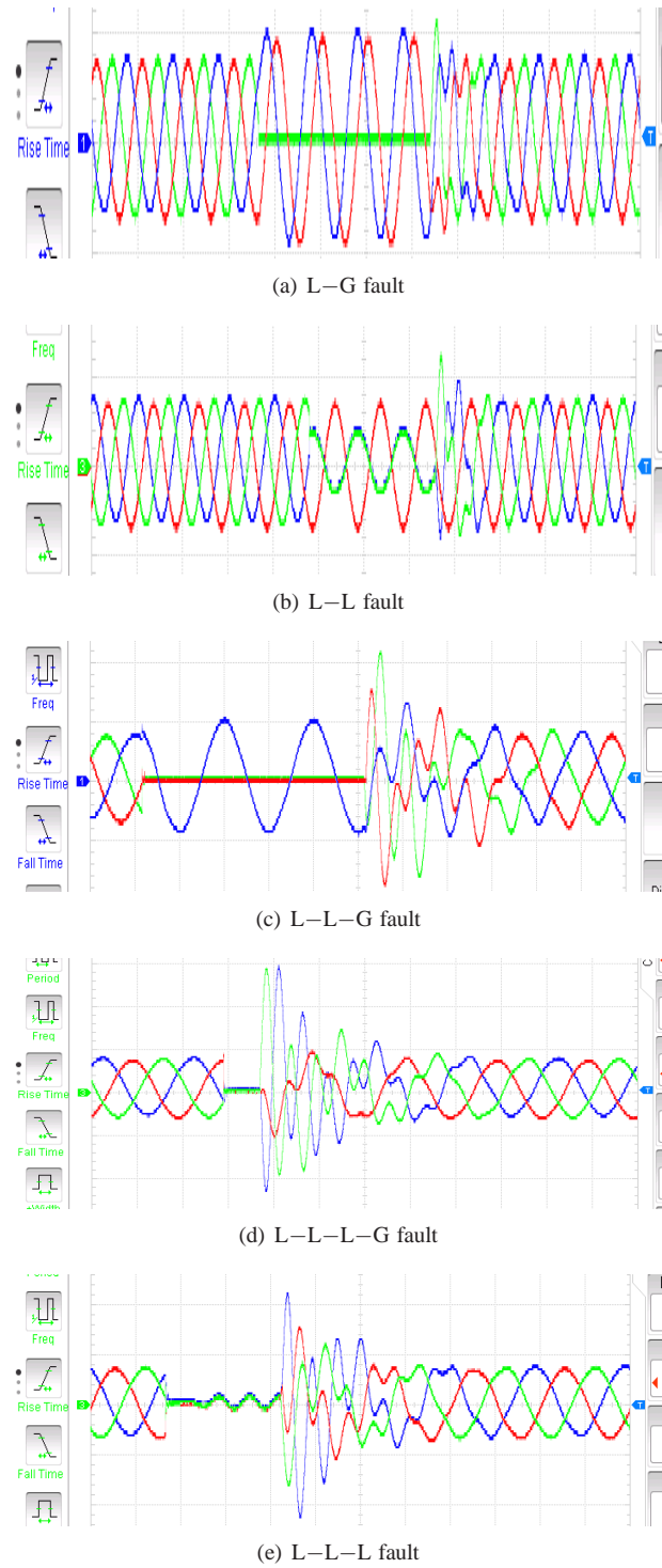
Fig. 11: Three phase real voltage signals fault
