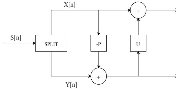
Fig. 2: Block diagram representation of SGWT decomposition
