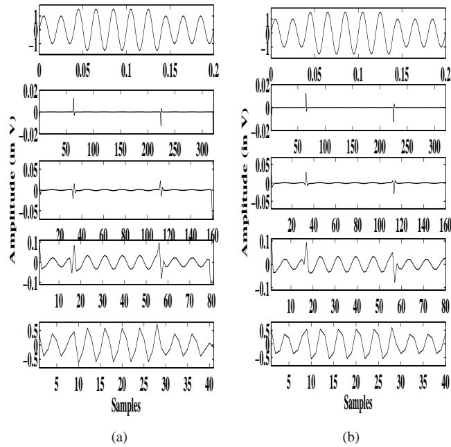
Fig. 5: Localization of sine wave with swell in (a) DWT decomposition (b) SGWT decomposition
