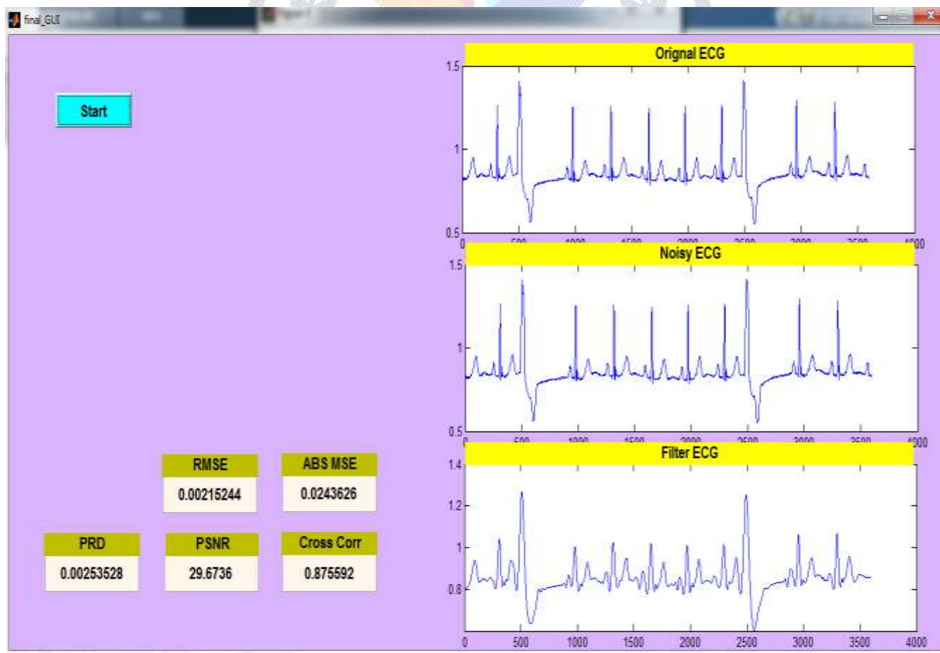
Figure 4 GUI developed for user interface
