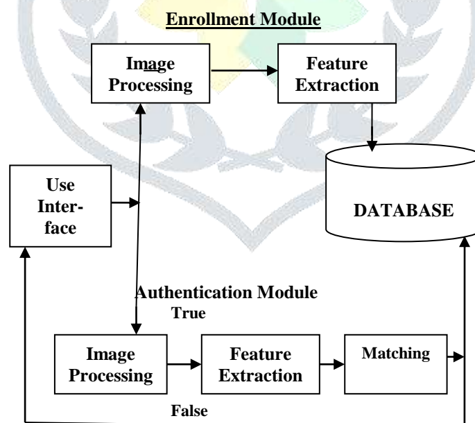
Fig 1: Process for handwriting verifier
