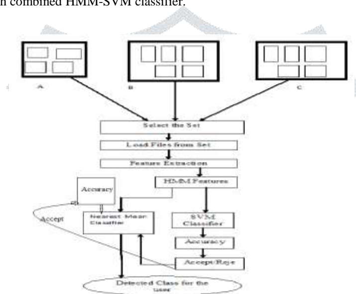
Fig 4: new approach Of HMM-SVM
