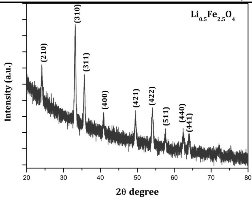
Fig. 2 The X-ray diffraction pattern of lithium ferrite thin film
