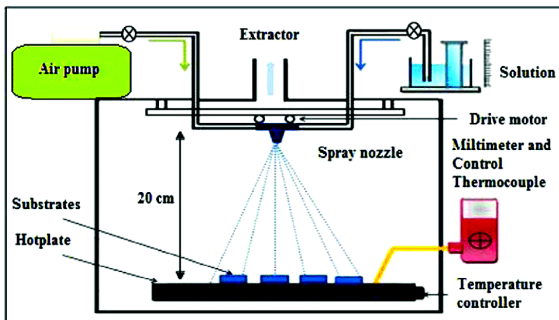
Fig. 1 Schematic of spray deposition
