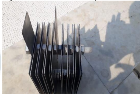
Fig 1. Electrolytic plates configuration
