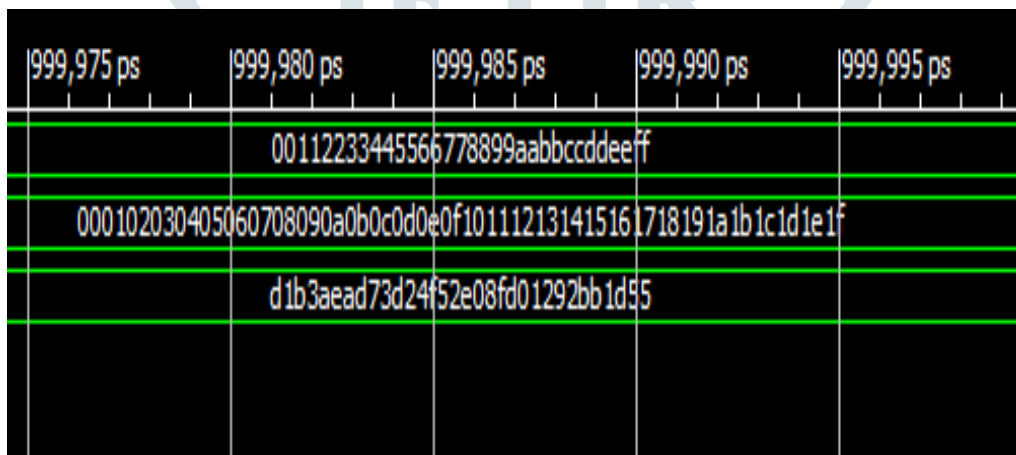
Figure 5: Encryption Process
