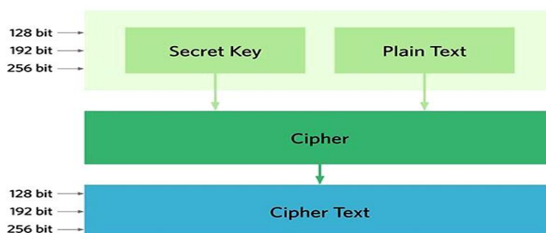
Figure 1: AES Model
