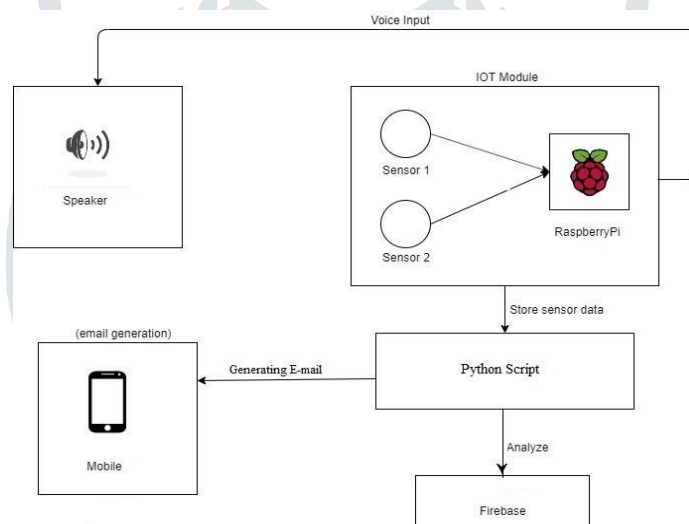
Fig. 5 System Architecture
