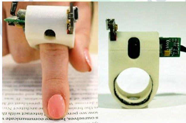
Fig 3.Finger Reader
