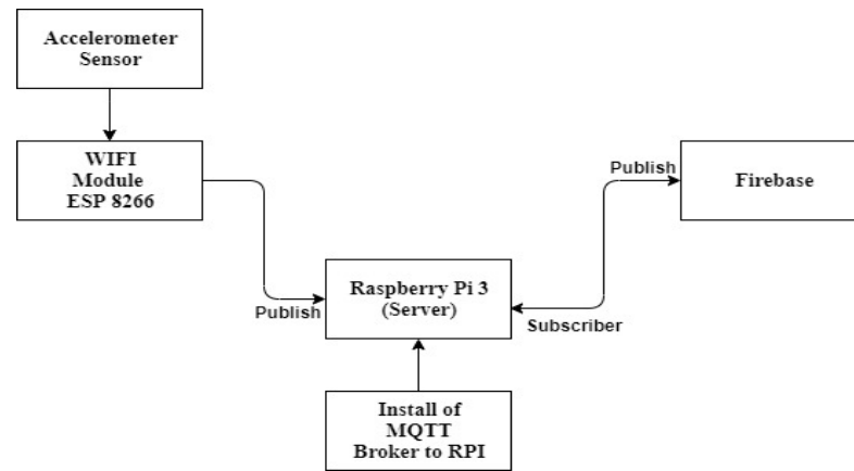
Fig 6:Proposed System
