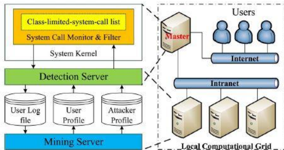
Fig 1. System Architecture
