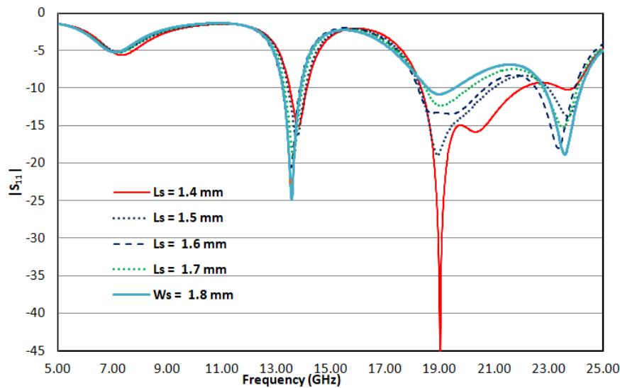
Fig 5: Return loss of antenna for variation in ground plane
