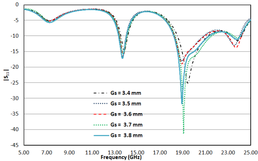
Fig 4: Return loss of antenna for variation in slot
