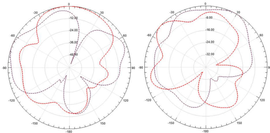
Fig. 8 E-Field and H-Field Radiation pattern at 13.75GHz (Red: \theta=0^\circ ,Green: \Phi=90^\circ )
