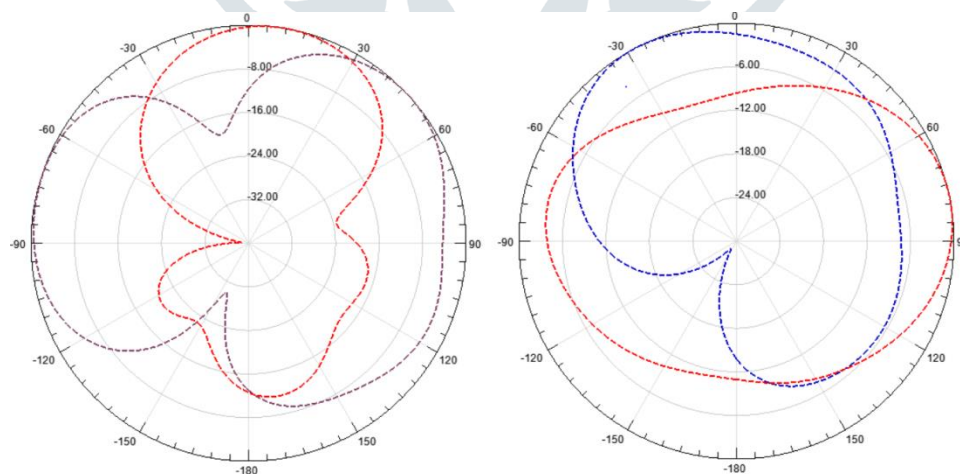
Fig. 6 E-Field and H-Field Radiation pattern at 13.75 GHz (Red : \theta=0^\circ , Green: \Phi=90^\circ )
