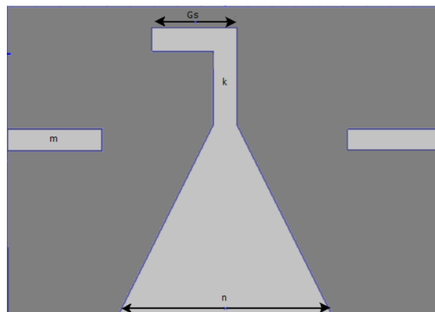
Figure 2. Proposed antenna design (Ground)
