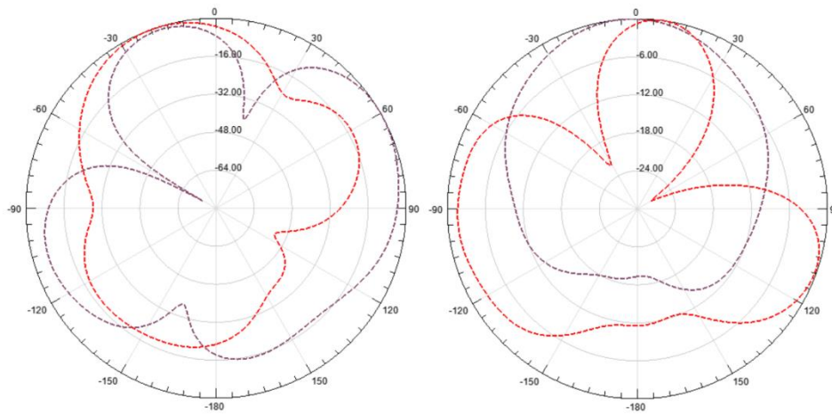
Fig. 7 E-Field and H-Field Radiation pattern at 19.0GHz (Red: \theta=0^\circ ,Green: \Phi=90^\circ )
