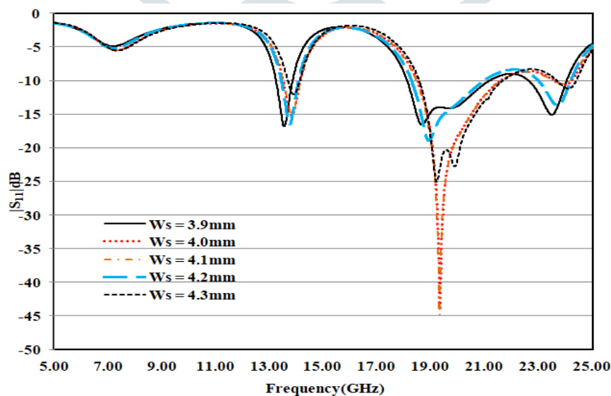
Fig 3: Return loss of antenna for variation in slot
