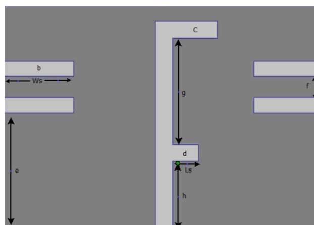
Figure 1. Proposed antenna design (Patch)
