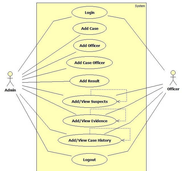
b) Use Case Diagram
