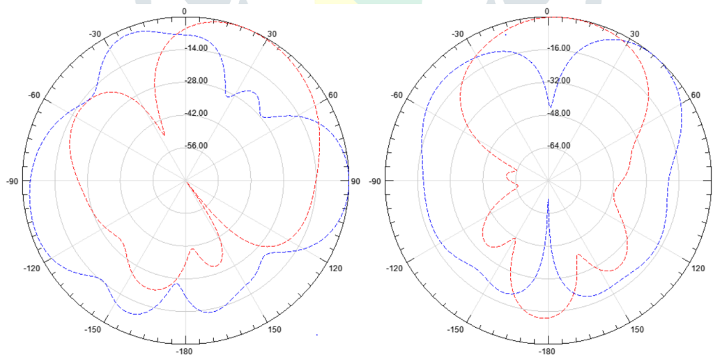
Fig. 8 E-Field and H-Field Radiation pattern at 7.51 GHz (Red: \theta=0^\circ ,Green: \Phi=90^\circ )
