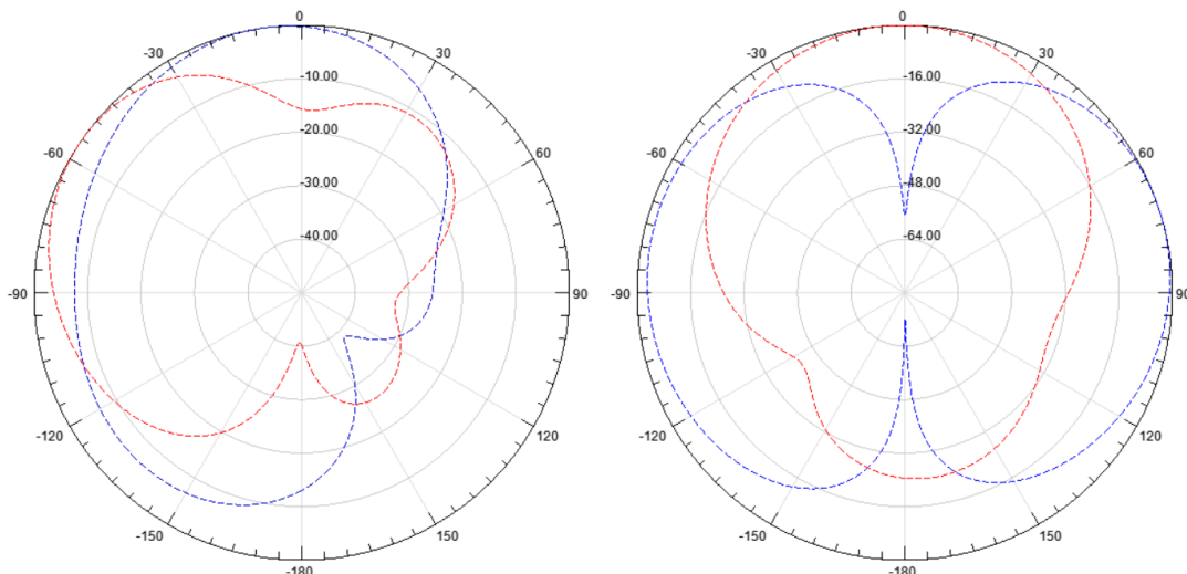
Fig. 5 E-Field and H-Field Radiation pattern at 2.2 GHz (Red : \theta=0^\circ ,Green: \Phi=90^\circ )
