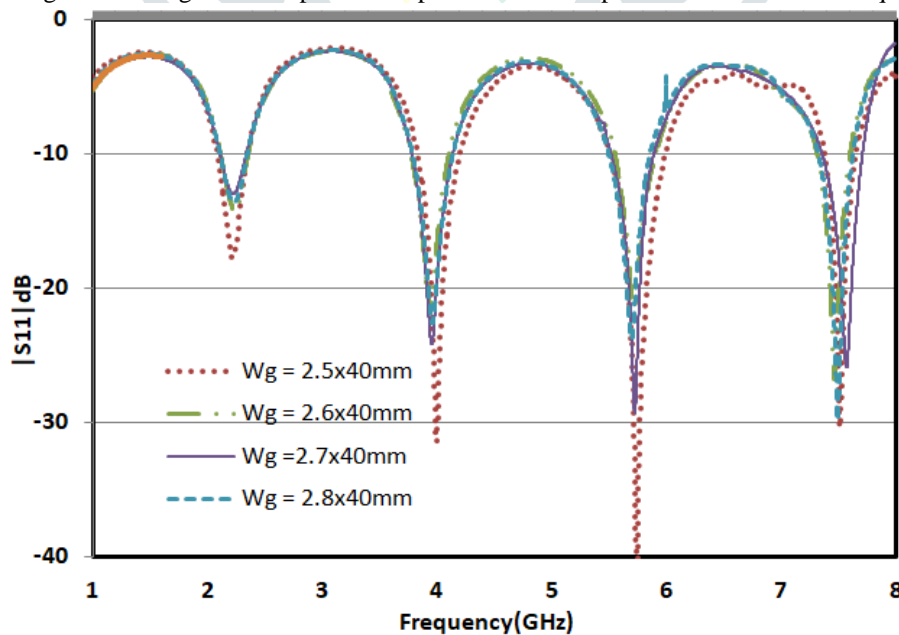
Fig 2: Return loss of antenna for variation in slot
