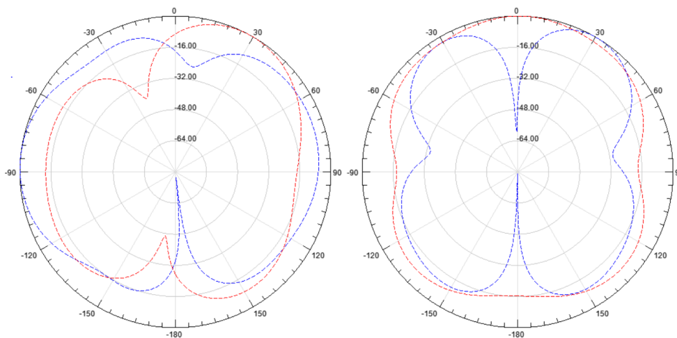
Fig. 6 E-Field and H-Field Radiation pattern at 4.0 GHz (Red: \theta=0^\circ ,Green: \Phi=90^\circ )
