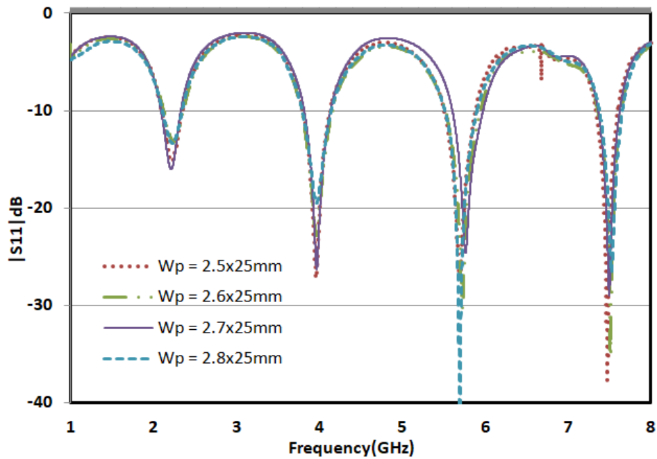
Fig 3: Return loss of antenna for variation in slot
