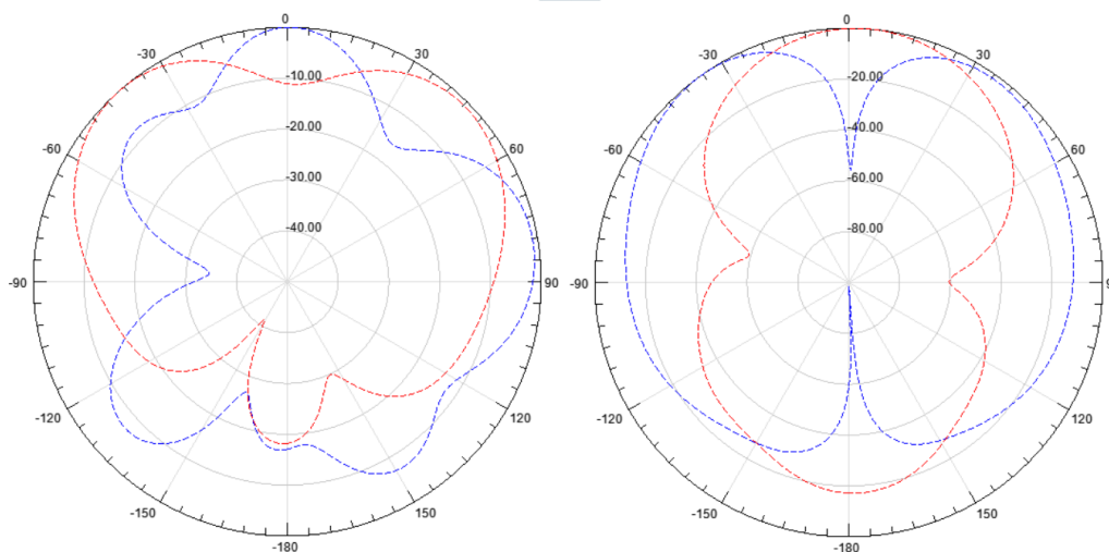
Fig. 7 E-Field and H-Field Radiation pattern at 5.75 GHz (Red: \theta=0^\circ ,Green: \Phi=90^\circ )
