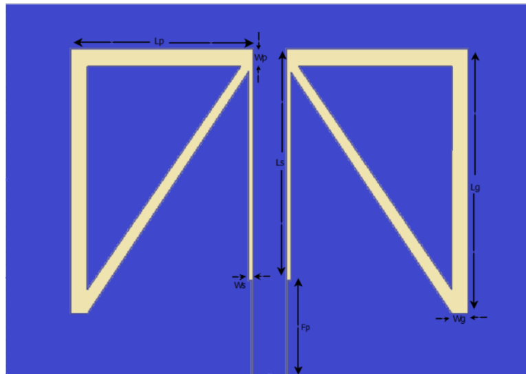
Figure 1. Proposed antenna design (Patch)
