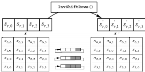
Fig: F-Inverse shift row transformation
