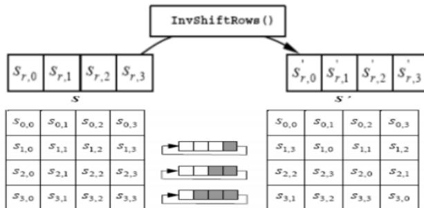
Fig: C-Shift row transformation
