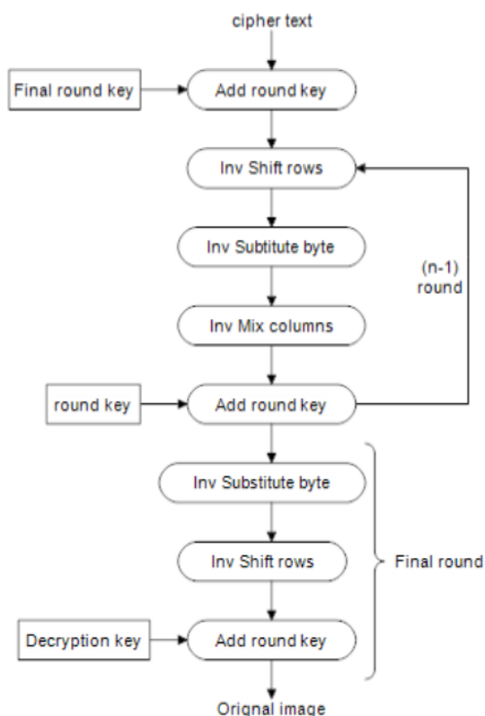
Fig: I-Decryption Algorithm
