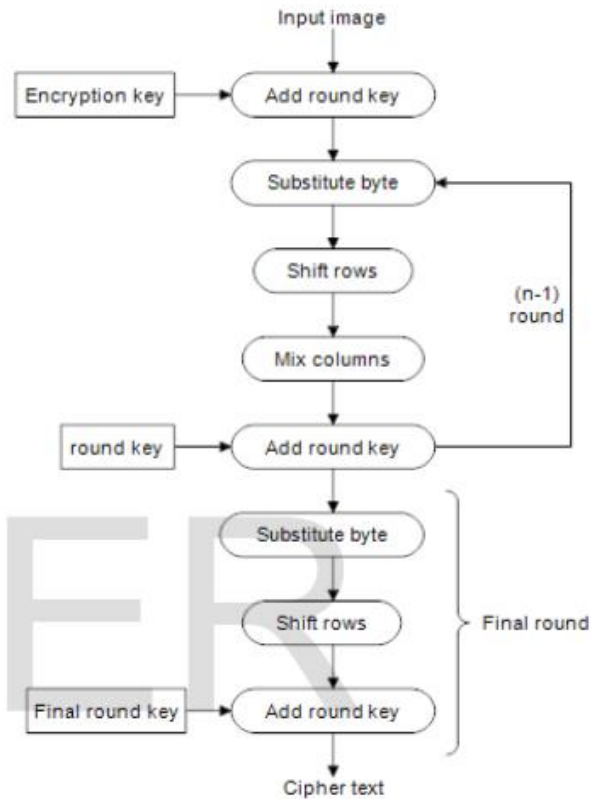
Fig: H-Encryption Algorithm
