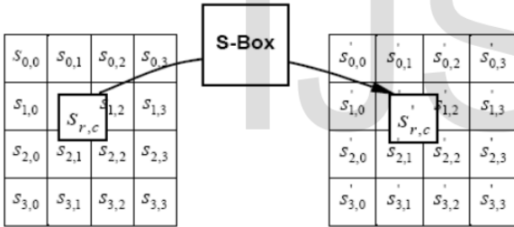
Fig: B-Substitute by transformation
