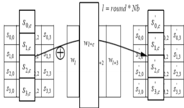
Fig: E-Round key transformation
