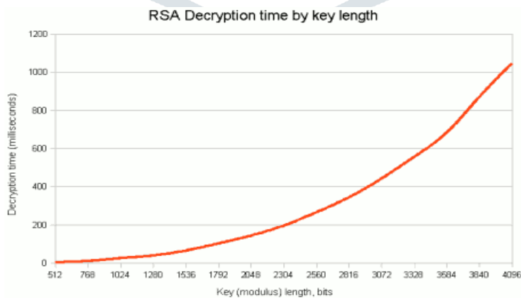
Figure 6 : Decryption time-image size
