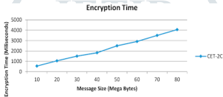
Figure 5 : Encryption time-image size
