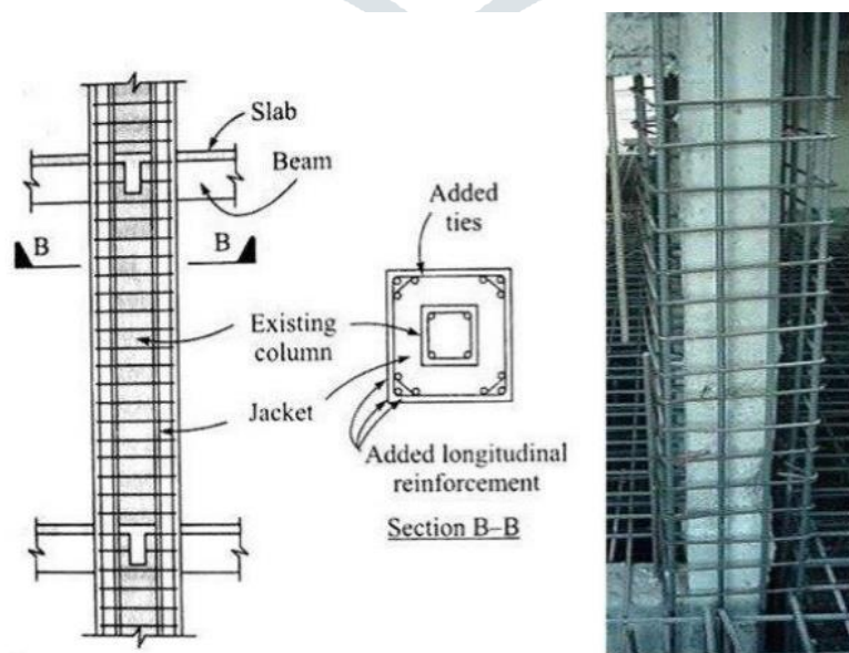
Fig 1.4. Column Jacketing
