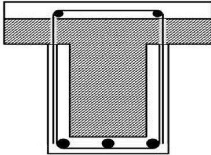
Fig 1.5. Beam Jacketing
