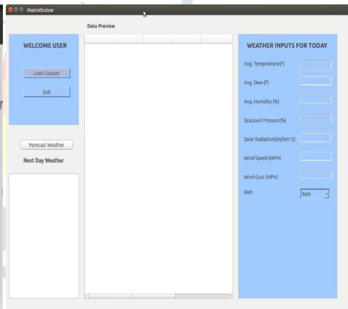
Fig 4. Home Page
