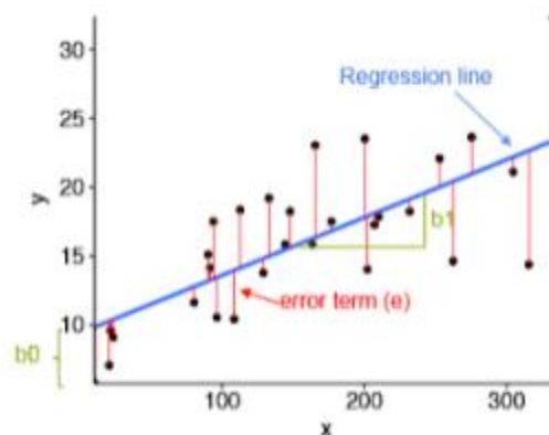
Fig.2. Regression Analysis
