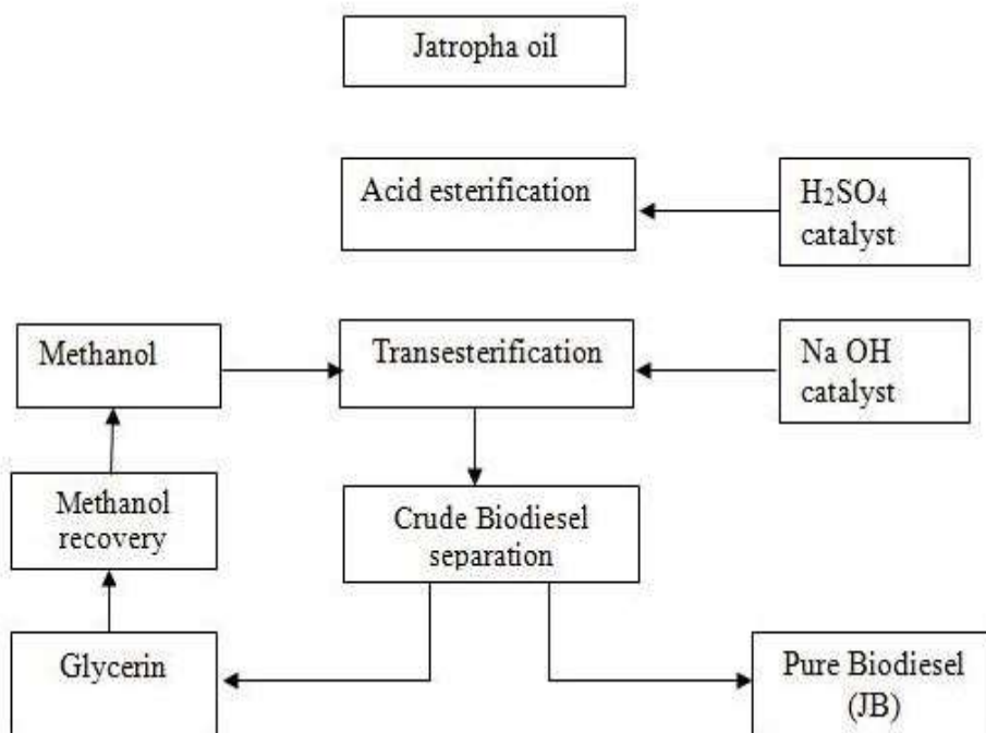
Fig.1 Transesterification Process.
