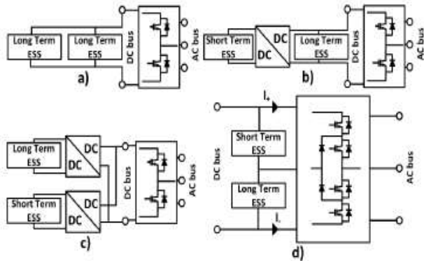
Fig.3.1. Power converter topologies for microgrid ESS hybridization (a) Passive (b) floating (c) parallel (d) 3L-NPC topology.
