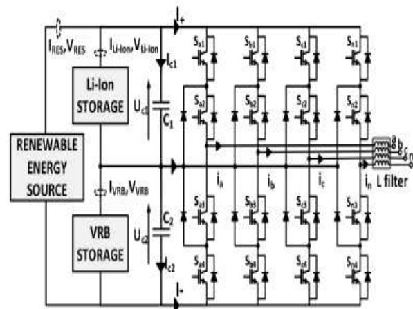
Fig.3.2. 4-Leg 3L-NPC topology used as a HESS/RES interface.
