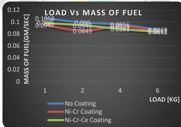
Graph 3:-Load Vs Mass of Fuel
