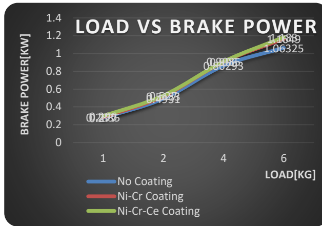
Graph 1:-Load Vs brake power
