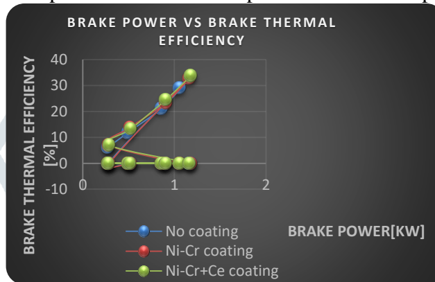
Graph 5:-Brake power Vs brake thermal efficiency
