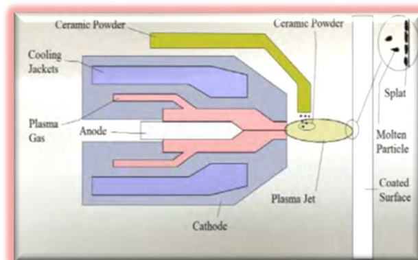
Fig 01: internal structure
