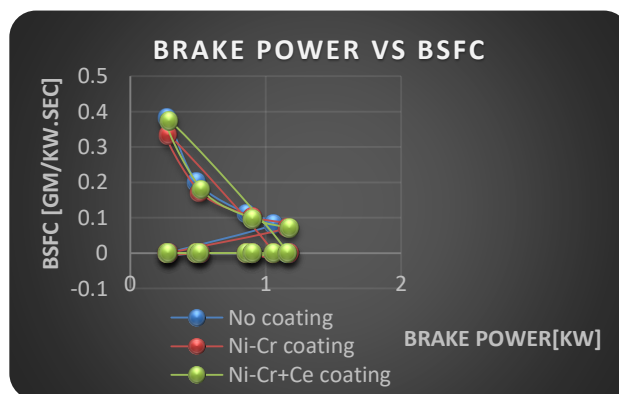
Graph 7:-Brake power Vs brake specific fuel consumption
