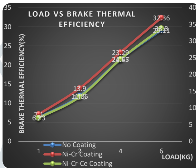
Graph 2:-Load Vs brake thermal efficiency
