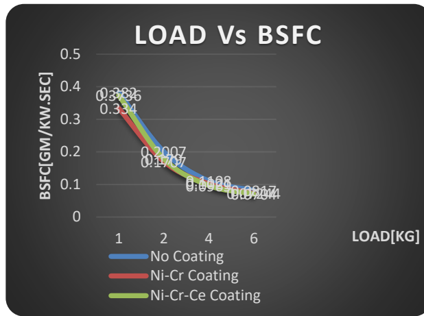
Graph 4:-Load Vs brake specific fuel consumption
