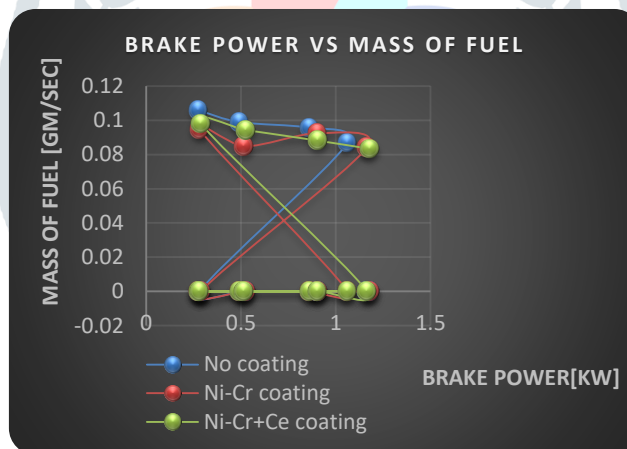
Graph 6:-Brake power Vs Mass of fuel
