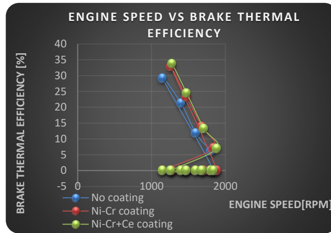
Graph 8:-Engine Speed Vs brake thermal efficiency
