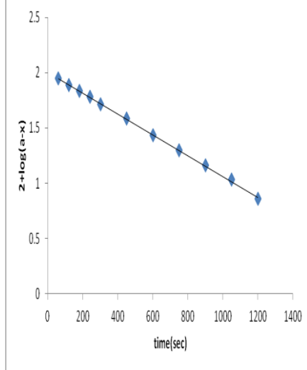
Figure 1. – Oxidation of Thiomalic acid by PiCC: A typical Kinetic Run
