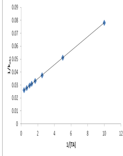
Figure 2. – Oxidation of Thiolactic acid by PiCC: A double reciprocal plot
