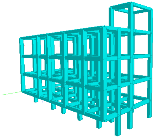
Fig. 3: 3-D view in STAAD.Pro with floating column at Edge column position
