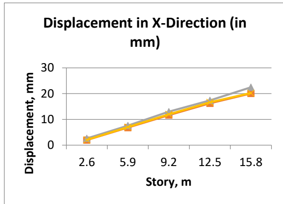
Fig. 5: Maximum displacements of the floating column at X-Direction
