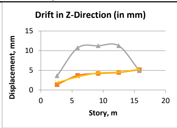
Fig. 8: Maximum Story drift of the floating column at Z-Direction
