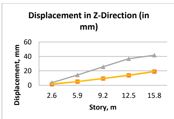
Fig. 6: Maximum displacements of the floating column at Z-Direction
