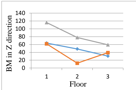
Fig. 11: comparison graph of Bending moment for all models
