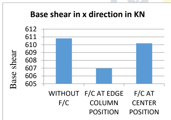
Fig. 9: Base shear at X-Direction
