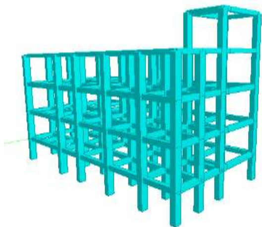
Fig. 4: 3-D view in STAAD.Pro with with floating column at Centre portion
