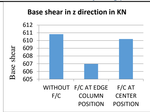
Fig. 10: Base shear at Z-Direction
