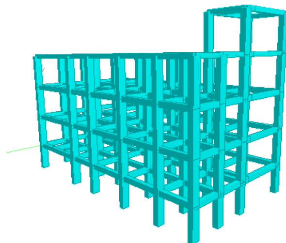
Fig. 2: 3-D view in STAAD.Pro without floating column
