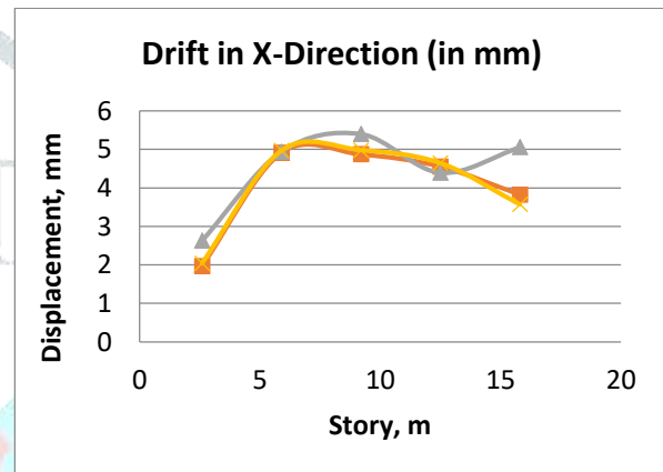
Fig. 7: Maximum Story drift of the floating column at X-Direction
