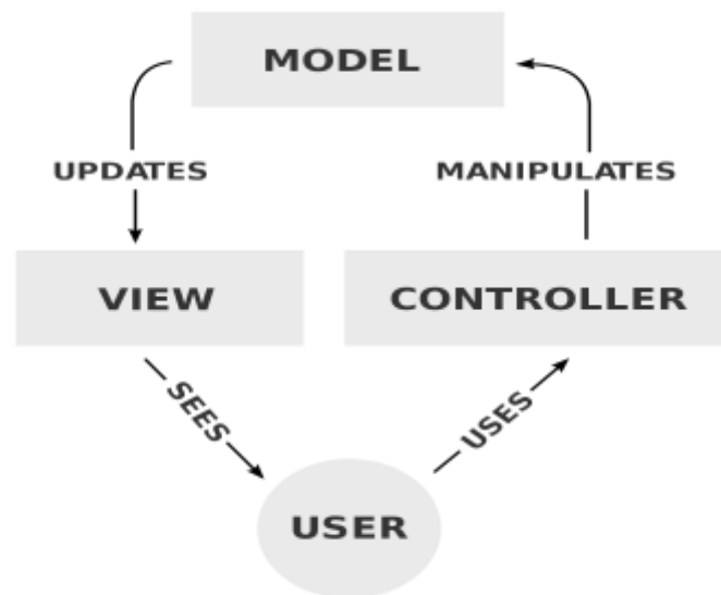
Fig2. MVC Architecture
